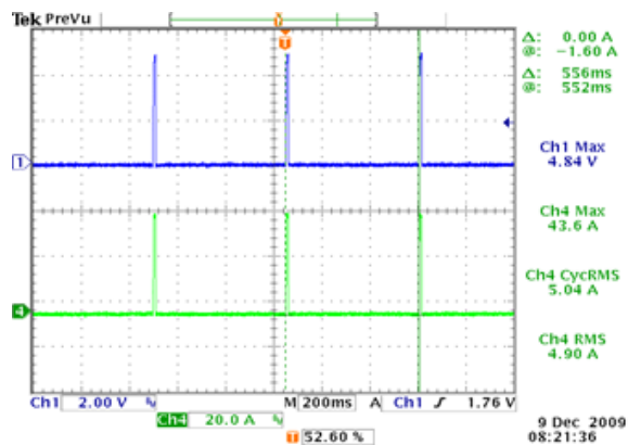
Figure 17. V_{in}=48V , V_{out}=5V , R_{out}=0.09\Omega
