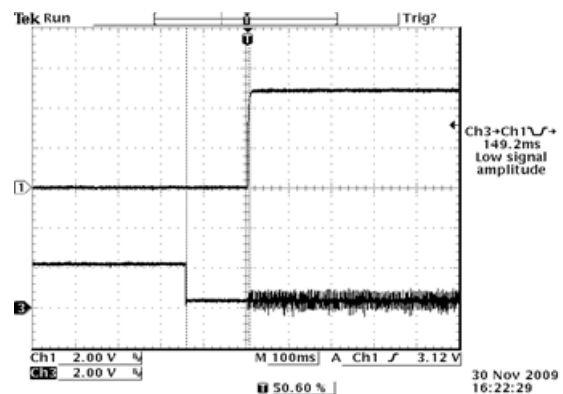
Figure 10. Startup from onn/off Ch1: V_o Ch2: V_{in} V_{in}=48V , V_o=5V , I_o=30A
