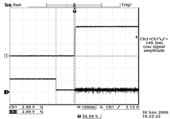
Figure 8. Startup from onn/off Ch1: V_o Ch2: V_{in} V_{in}=24V , V_o=5V , I_o=30A
