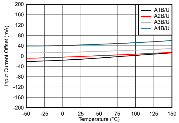
Figure 7-2. TMCS1108-Q1 Input Offset Current vs. Temperature
