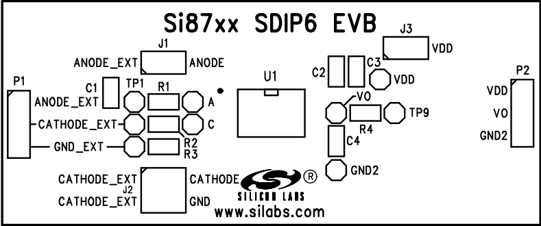
Figure 8. Si87xx SDIP6 Evaluation Board Silkscreen
