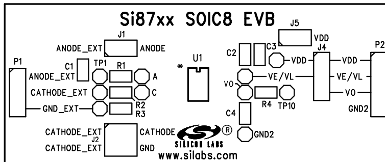
Figure 7. Si87xx SOIC8 Evaluation Board Silkscreen
