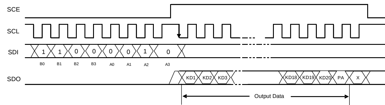
Figure 16. Serial Data Output Format
