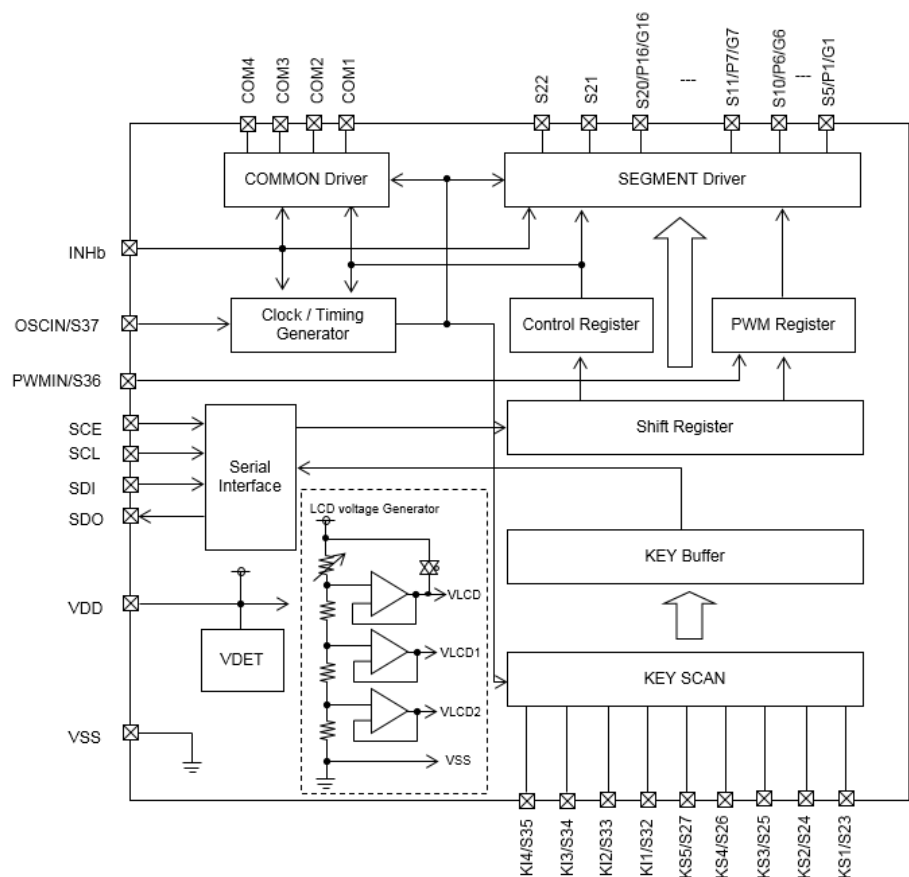
Figure 2. Block Diagram
