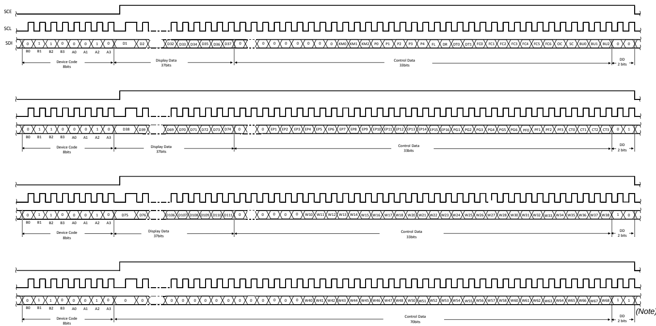
Figure 9. 3-SPI Data Transfer Format
