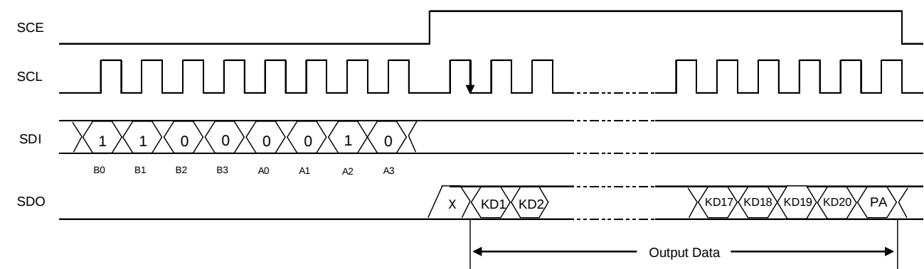
Figure 15. Serial Data Output Format
