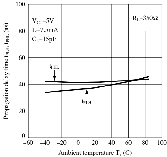
Fig.11-c Propagation Delay Time vs. Ambient Temperature
