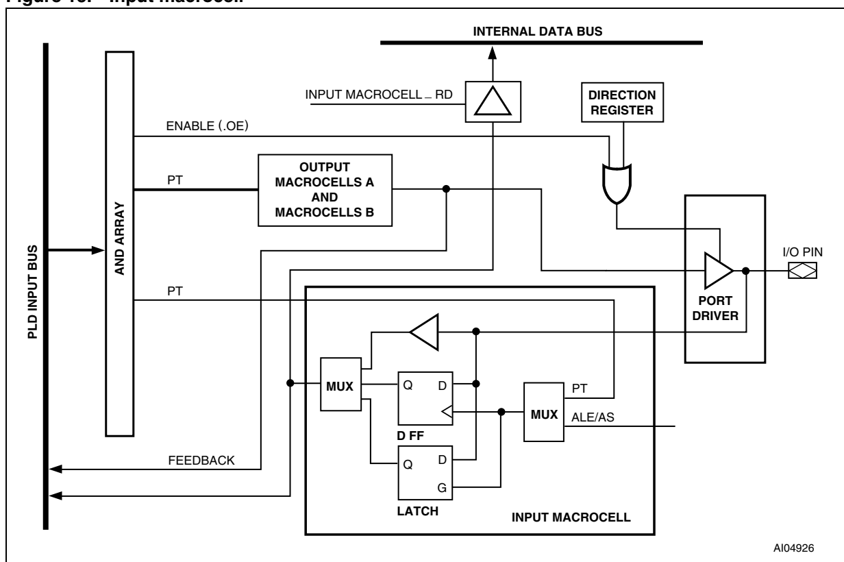
Figure 15. Input macrocell
