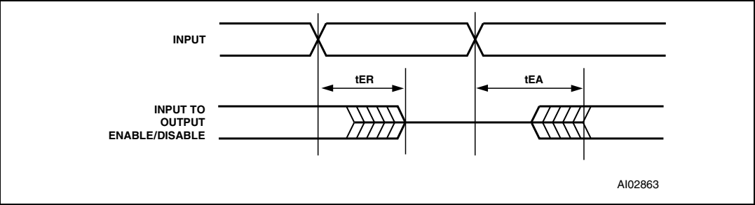
Figure 43. Input to Output Disable / Enable
