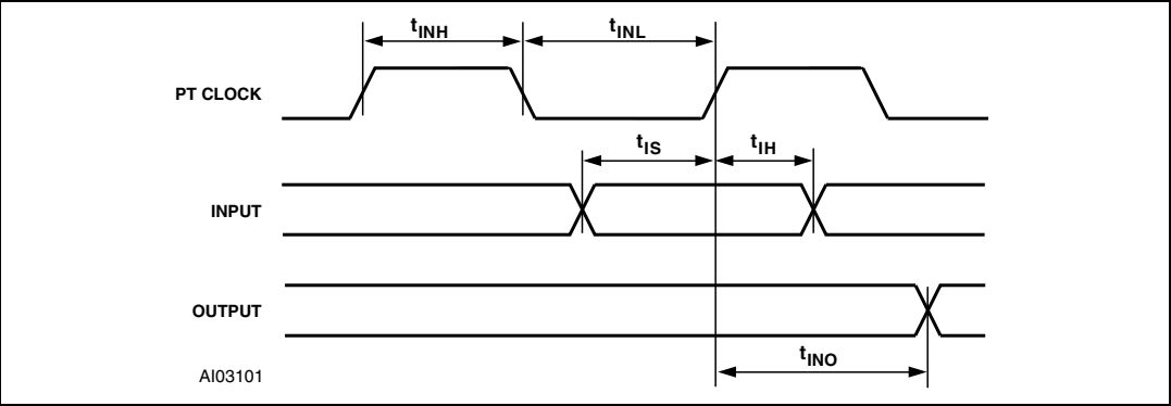
Figure 47. Input macrocell timing (Product Term Clock)
