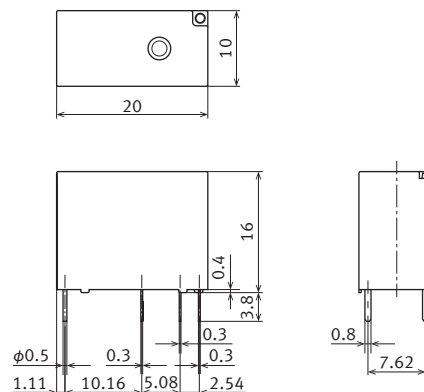
External dimensions
