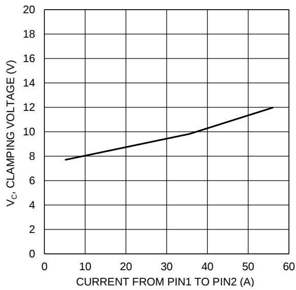
Figure 5 Clamping Voltage Characteristic ( t_p=8/20\mu s )
