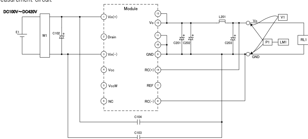
Measurement circuit
