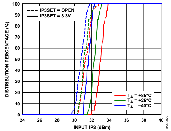
Figure 29. Input IP3
