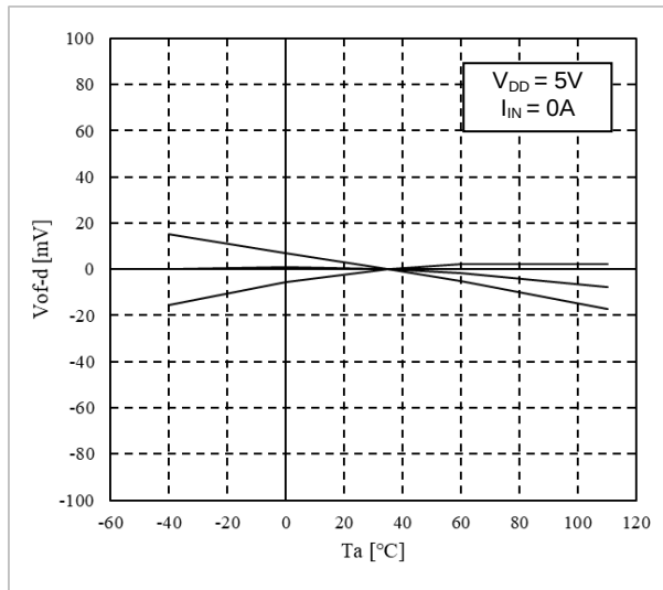
Figure 6. Temperature drift of offset voltage (for reference, n=3)
