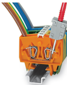
Testing via CAGE CLAMP® on the current bar (max. nominal current: 6 A). CAGE CLAMP® clamps individual test pins contacts. The maximum test voltage is 400 V.
