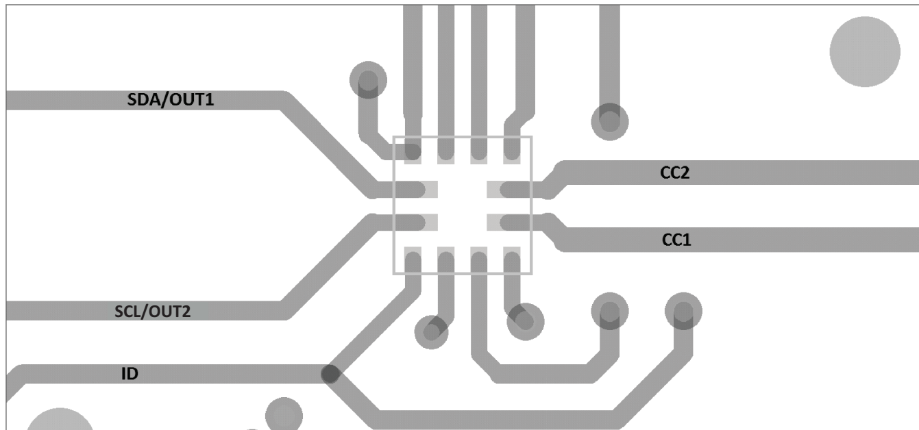
Figure 22. TUSB320 Layout
