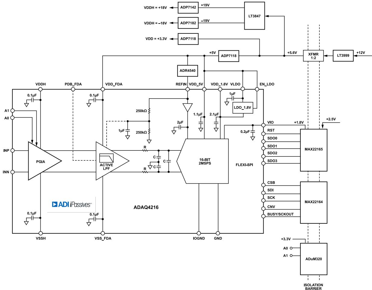
Figure 94. Functional Block Diagram of a Fully Isolated Data-Acquisition System
