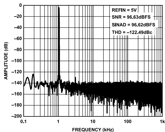
Figure 26. FFT, 2MSPS, f_{IN} = 1\text{kHz} , Differential Input = -0.5\text{dBFS} , G = 20/3 , \text{REFIN} = 5\text{V}
