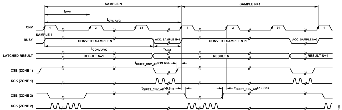
Figure 116. Example of Different Zones in Averaging Mode (64 Samples Averaged)
