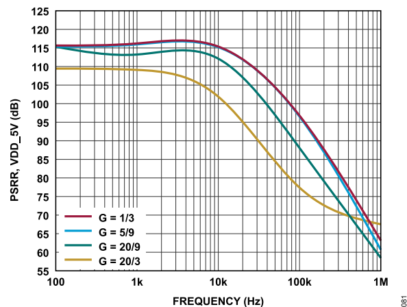
Figure 83. PSRR vs. Frequency, VDD_5V
