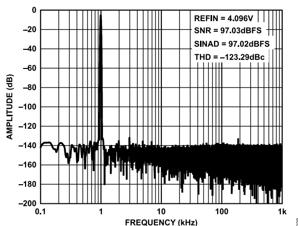
Figure 28. FFT, 2MSPS, f_{IN} = 1\text{kHz} , Differential Input = -0.5\text{dBFS} , G = 20/9 , \text{REFIN} = 4.096\text{V}
