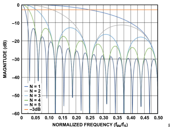
Figure 92. Frequency Response Examples for the Block Averaging Filter
