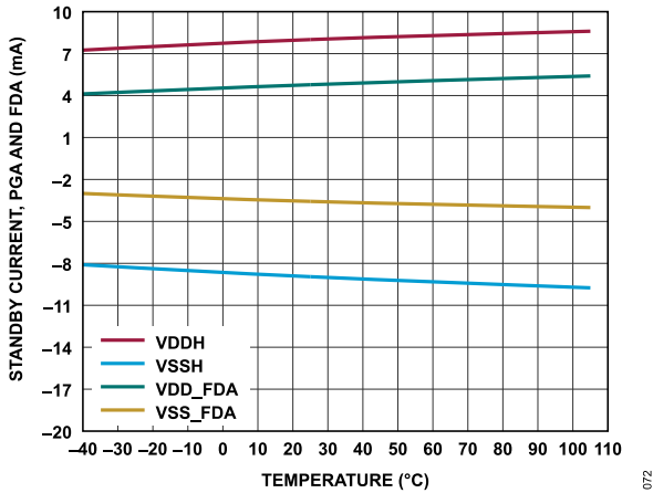
Figure 72. Standby Current PGA and FDA vs. Temperature
