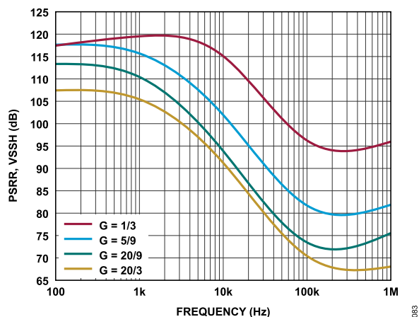
Figure 85. PSRR vs. Frequency, V_{SSH}
