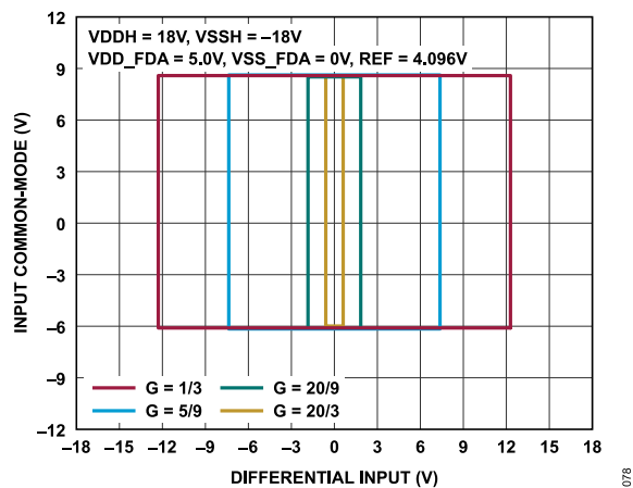
Figure 78. Input Common-Mode Voltage vs. Differential Input Voltage, REFIN = 4.096V, All Gains
