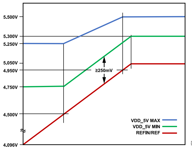
Figure 107. VDD_5V Minimum and Maximum Values for REFIN
