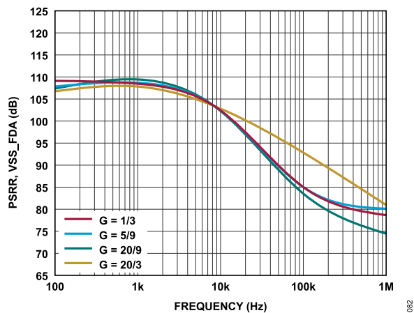
Figure 84. PSRR vs. Frequency, V_{SS\_FDA}
