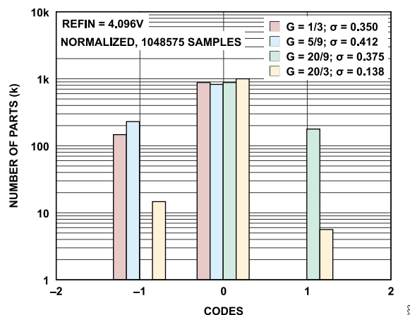
Figure 22. Code Histogram for Shorted Inputs, REFIN = 4.096V
