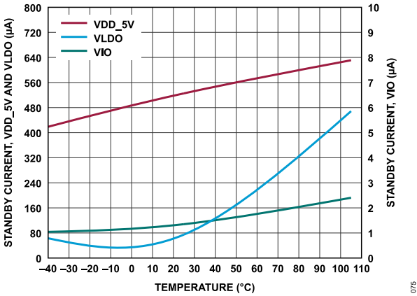
Figure 75. Standby Current ADC vs. Temperature
