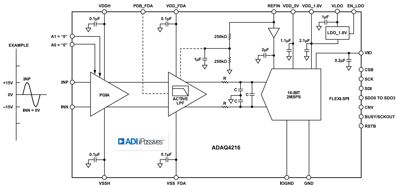
Figure 99. Single-Ended Input Configuration with G = 1/3V/V
