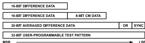
Figure 93. Summary of Selectable Output Sample Formats
