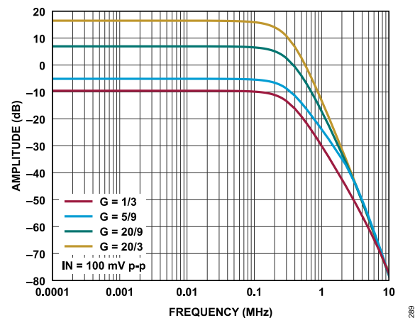
Figure 89. AAF Frequency Response
