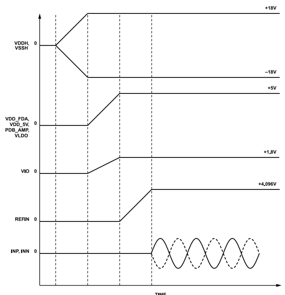
Figure 106. Power Supply Sequence
