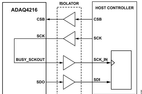
Figure 112. Echo Clock Mode Signal Path Diagram
