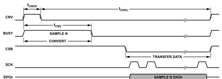
Figure 114. Basic Single Sample Conversion Cycle
