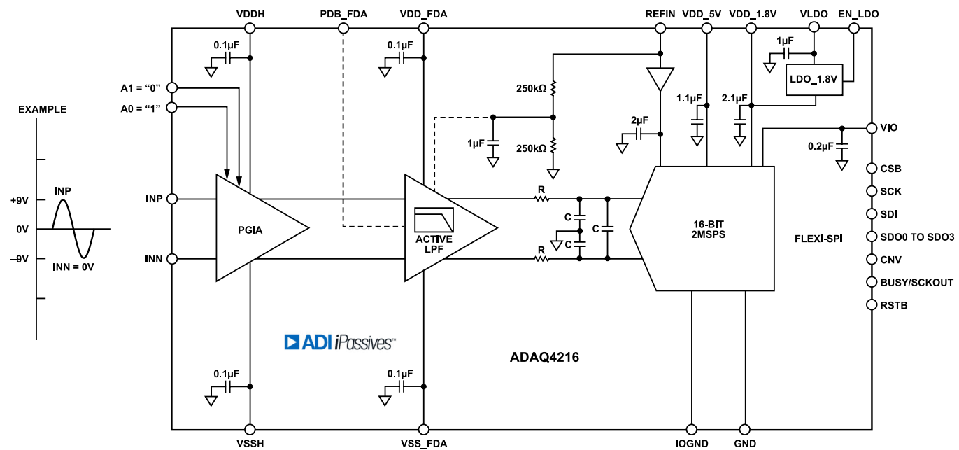
Figure 100. Single-Ended Input Configuration with G = 5/9V/V
