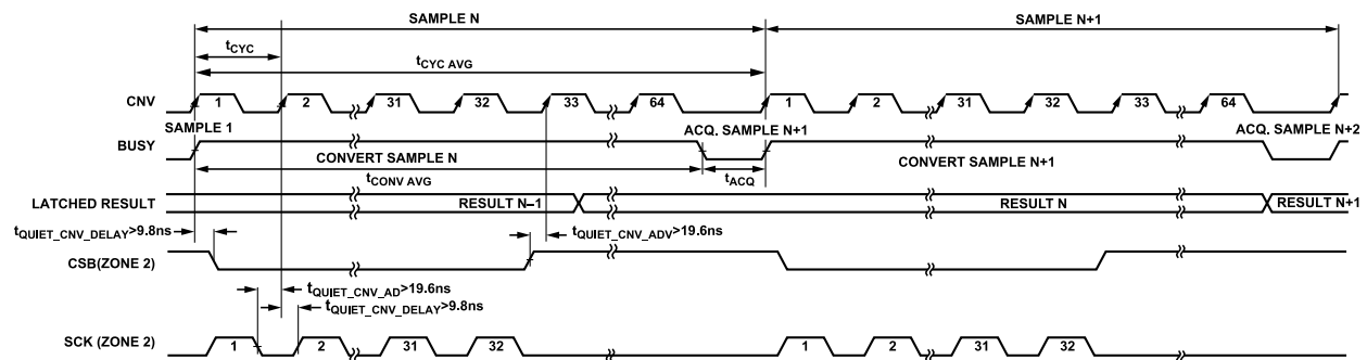
Figure 117. Example of Zone 2 in Averaging Mode (1 Bit per Sample)
