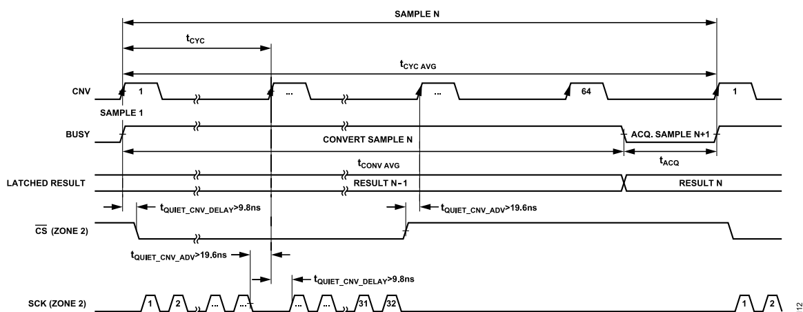
Figure 118. Example of Zone 2 in Averaging Mode (N Bits per Cycle)
