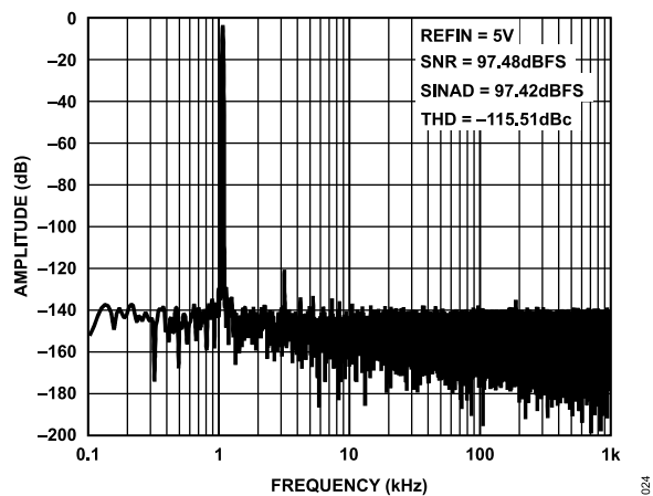
Figure 24. FFT, 2MSPS, f_{IN} = 1\text{kHz} , Differential Input = -0.5\text{dBFS} , G = 5/9 , \text{REFIN} = 5\text{V}
