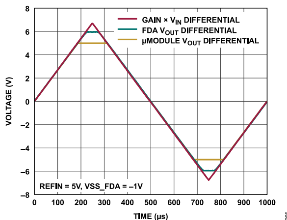
Figure 88. Output Overdrive Recovery, IN = 1\text{ kHz}
