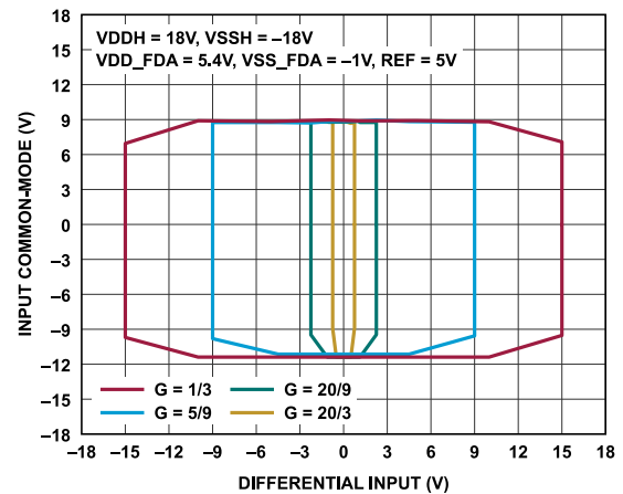
Figure 77. Input Common-Mode Voltage vs. Differential Input Voltage, REFIN = 5V, All Gains
