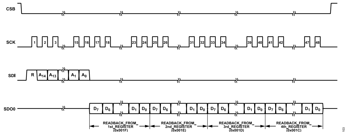
Figure 109. Stream Mode Bulk Register Readback Operation
