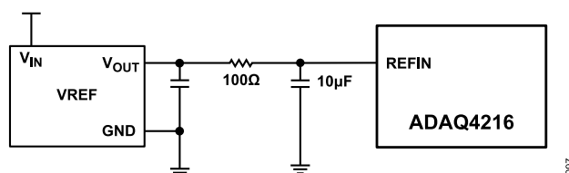
Figure 103. Reference with Noise Filter
