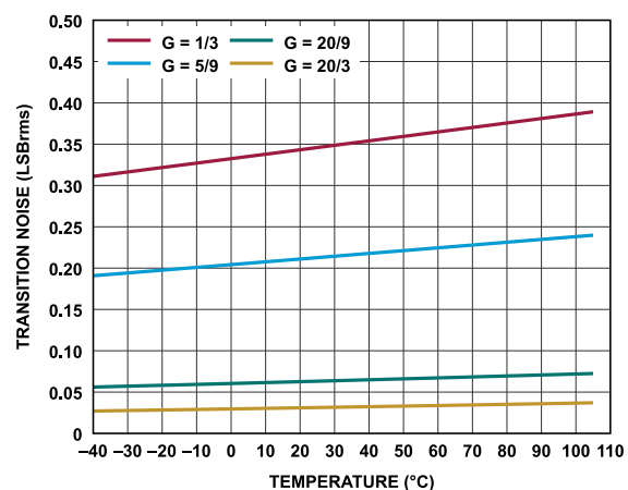
Figure 53. Transition Noise vs. Temperature, REFIN = 4.096\text{V}
