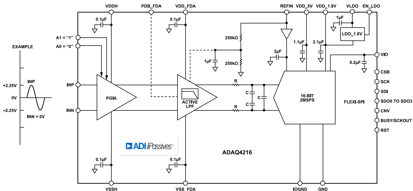
Figure 101. Single-Ended Input Configuration with G = 20/9V/V
