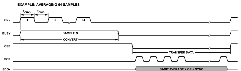
Figure 115. Example Conversion Cycle for Averaging Mode
