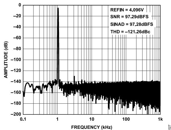
Figure 27. FFT, 2MSPS, f_{IN} = 1\text{kHz} , Differential Input = -0.5\text{dBFS} , G = 5/9 , \text{REFIN} = 4.096\text{V}
