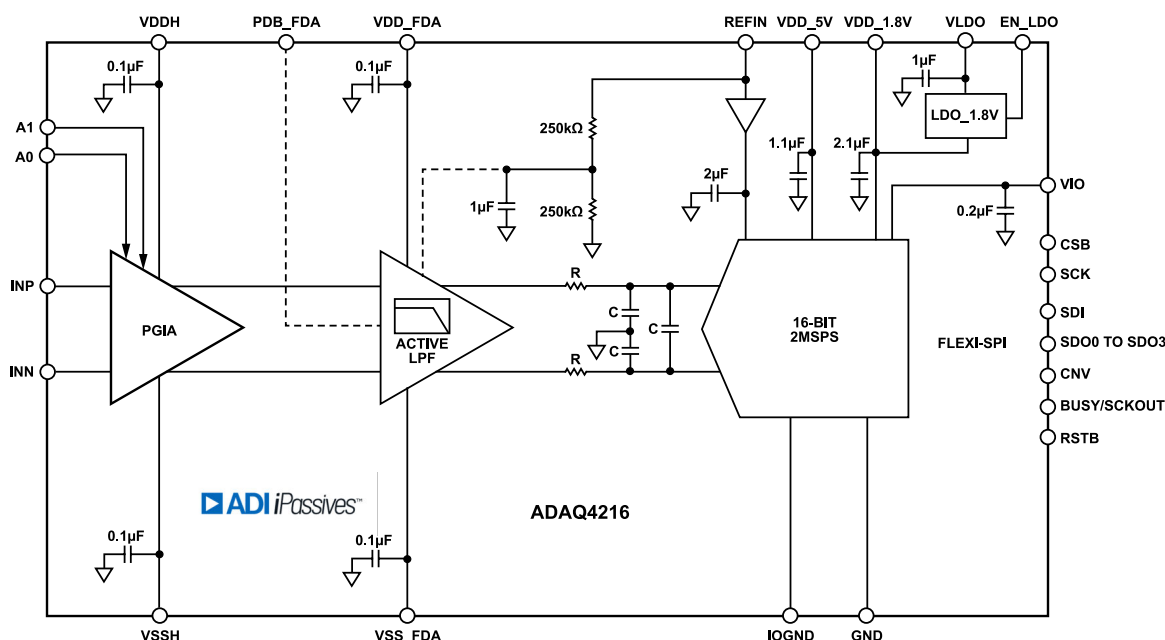
Figure 90. ADAQ4216 Functional Block Diagram
