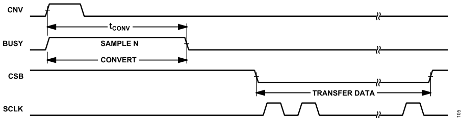
Figure 111. Typical Sample Cycle for SPI Clocking Mode
