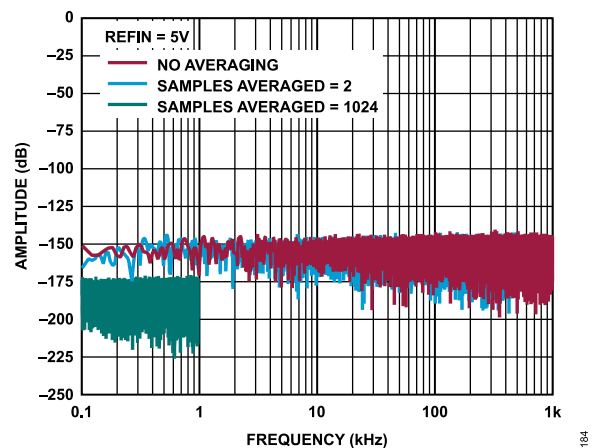
Figure 86. FFT, Grounded Inputs, REFIN = 5\text{ V}
