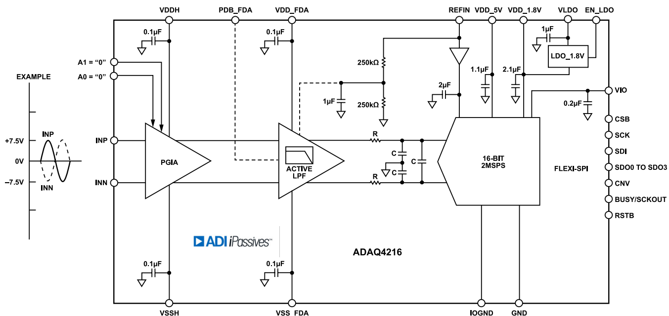
Figure 95. Differential Input Configuration with G = 1/3V/V
