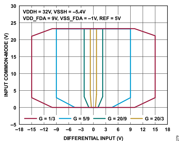
Figure 79. Input Common-Mode Voltage vs. Differential Input Voltage, VICM = Positive, All Gains
