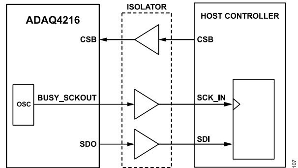
Figure 113. Host Clock Mode Signal Path Example
