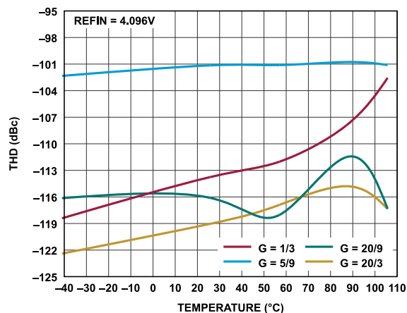
Figure 51. THD vs. Temperature, f_{IN} = 1\text{kHz} , Single-Ended Input, REFIN = 4.096\text{V}
