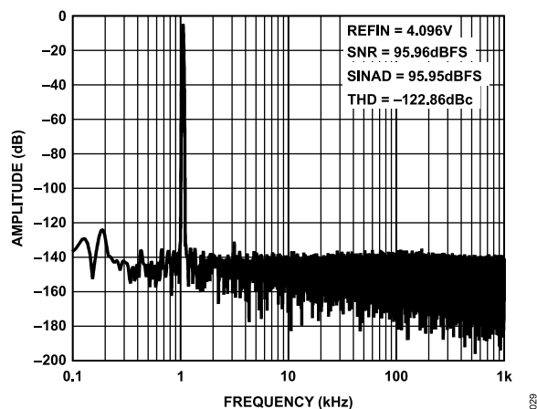
Figure 29. FFT, 2MSPS, f_{IN} = 1\text{kHz} , Differential Input = -0.5\text{dBFS} , G = 20/3 , \text{REFIN} = 4.096\text{V}
