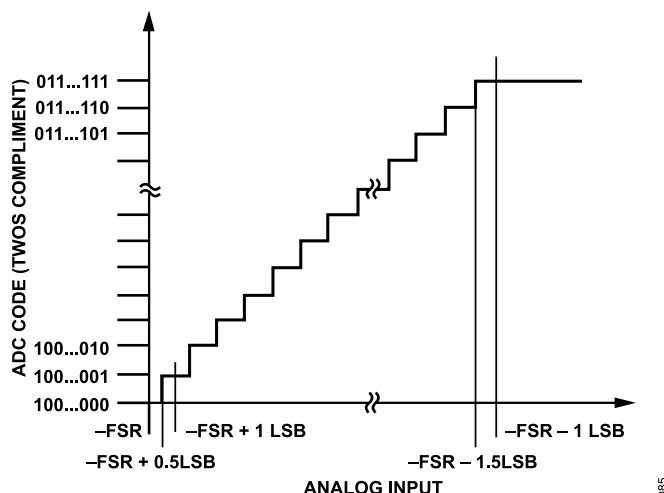
Figure 91. ADC Ideal Transfer Function for the Differential Output Codes (FSR Is Full-Scale Range)
