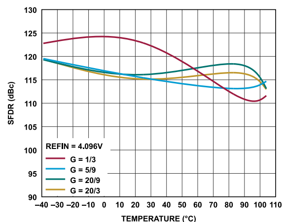
Figure 52. SFDR vs. Temperature, f_{IN} = 1\text{kHz} , REFIN = 4.096\text{V}
