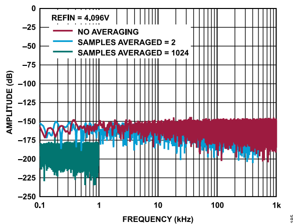
Figure 87. FFT, Grounded Inputs, REFIN = 4.096\text{ V}
