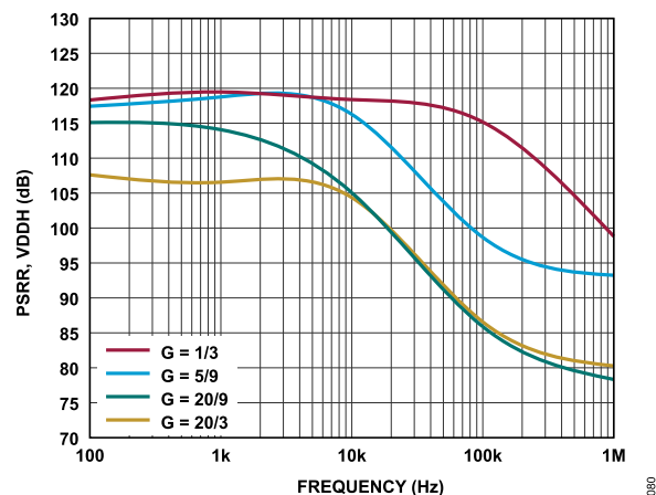
Figure 82. PSRR vs. Frequency, VDDH
