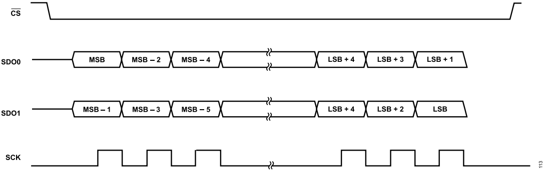
Figure 119. 2-Lane Mode, SDR Timing Diagram
