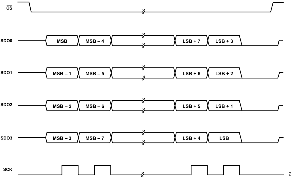
Figure 120. 4-Lane, SDR Timing Diagram
