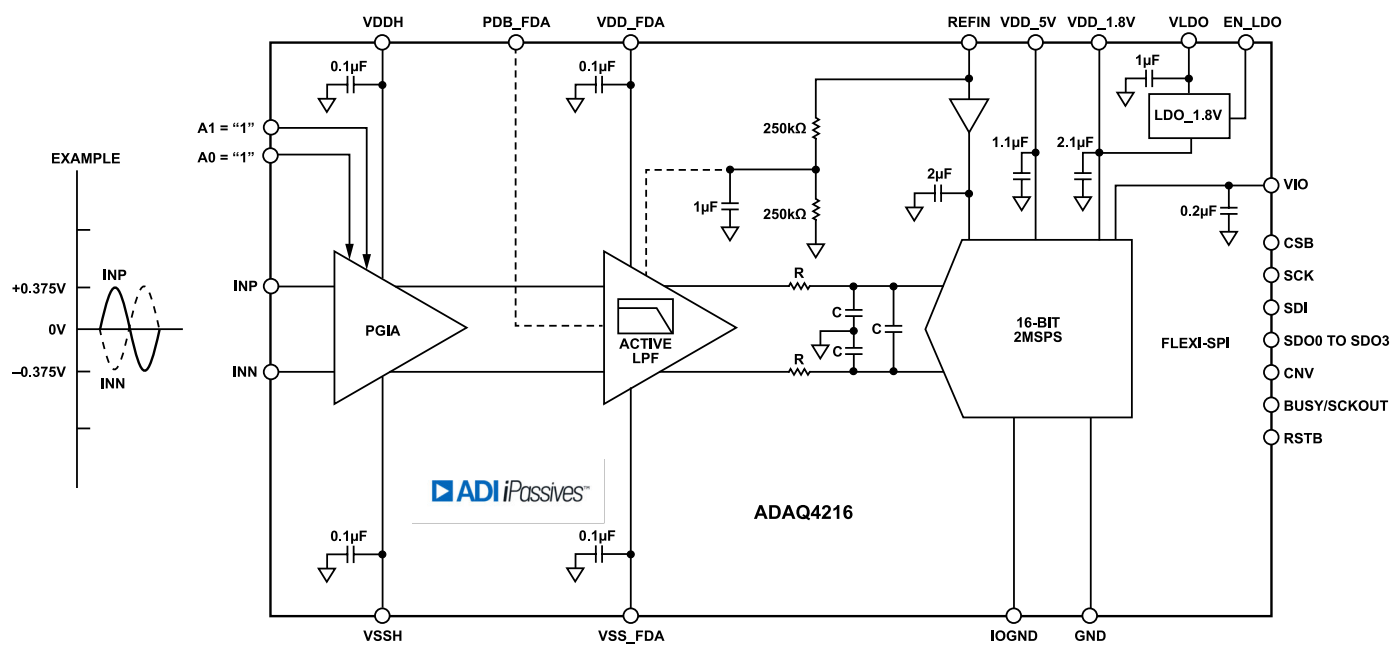
Figure 98. Differential Input Configuration with G = 20/3V/V
