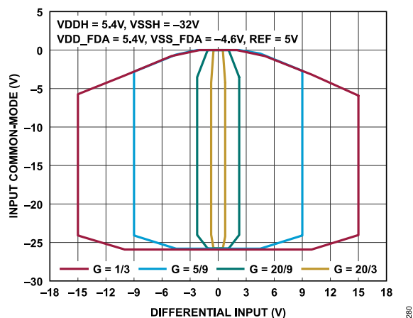
Figure 80. Input Common-Mode Voltage vs. Differential Input Voltage, VICM = Negative, All Gains
