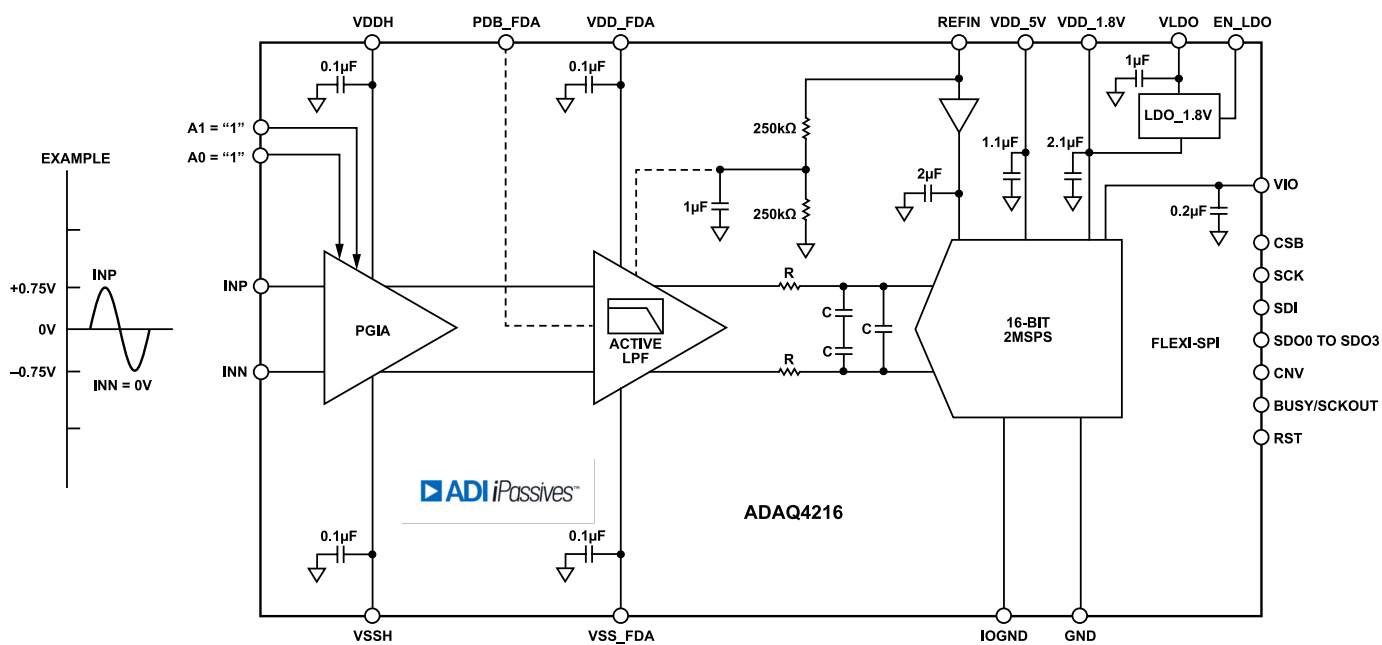
Figure 102. Single-Ended Input Configuration with G = 20/3V/V
