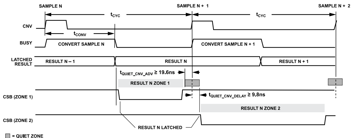
Figure 110. Example Timing for Data Transfer Zones
