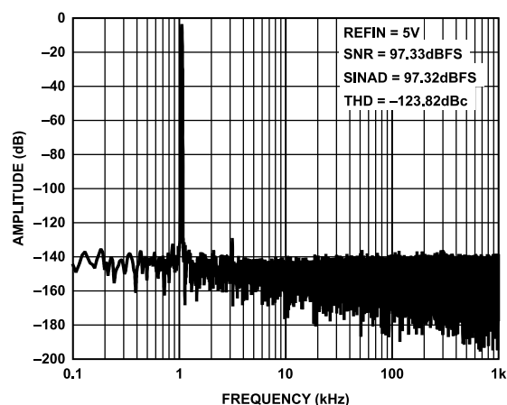
Figure 25. FFT, 2MSPS, f_{IN} = 1\text{kHz} , Differential Input = -0.5\text{dBFS} , G = 20/9 , \text{REFIN} = 5\text{V}
