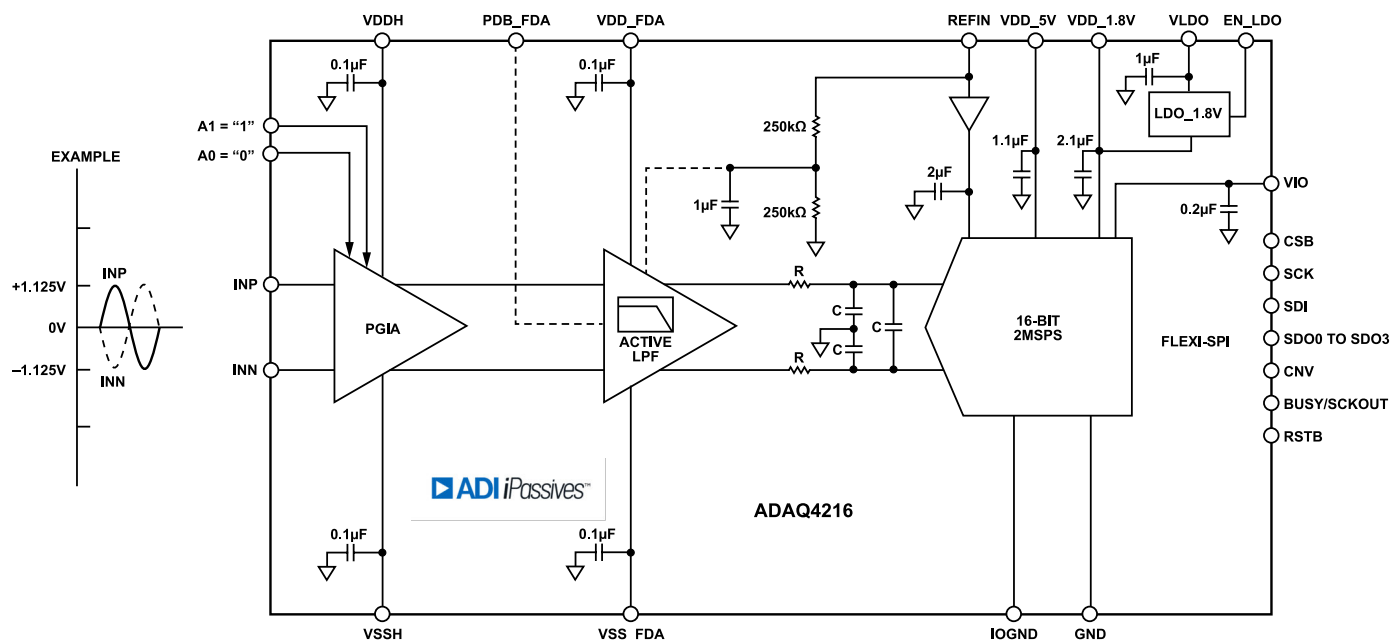
Figure 97. Differential Input Configuration with G = 20/9V/V
