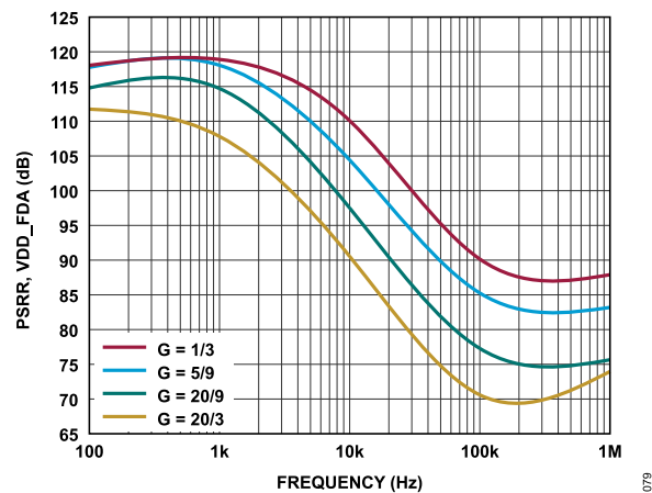
Figure 81. PSRR vs. Frequency, VDD_FDA
