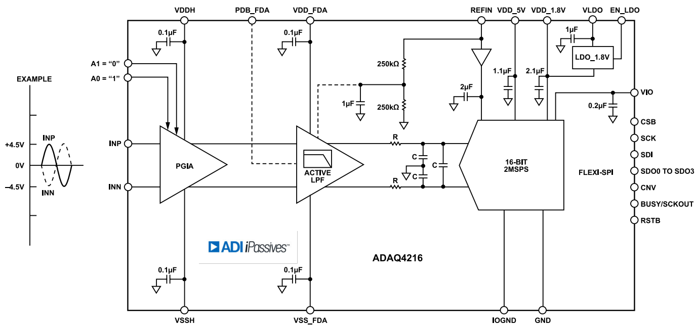
Figure 96. Differential Input Configuration with G = 5/9V/V
