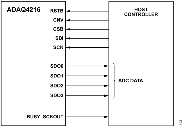
Figure 108. ADAQ4216 Multilane SPI
