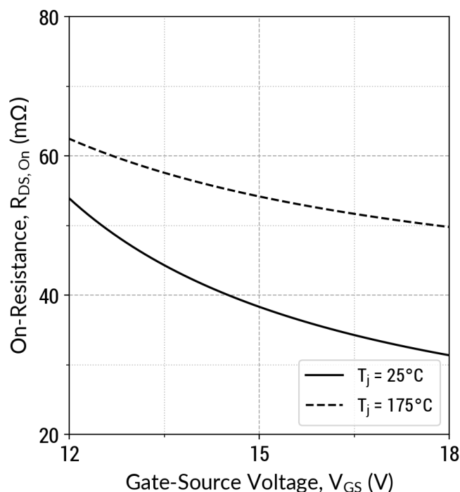
Figure 8: On-State Resistance v/s Gate Voltage
