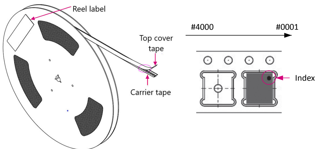
Figure 14. Component orientation
