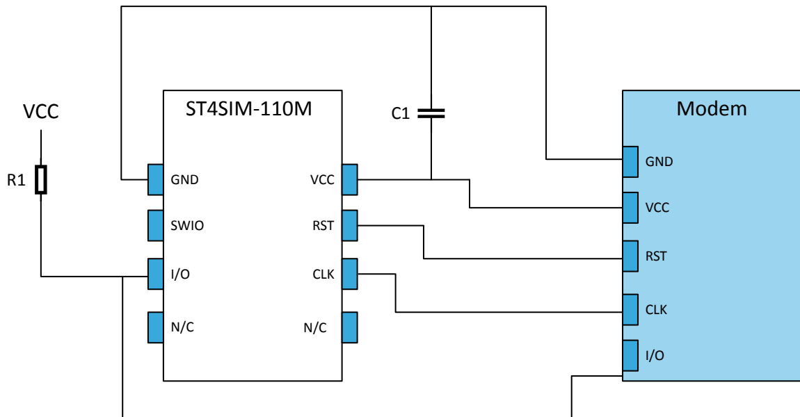
Figure 10. ST4SIM-110M PCB integration recommendations
