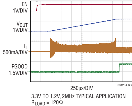
Start-Up Waveforms Pulse-Skipping Mode
