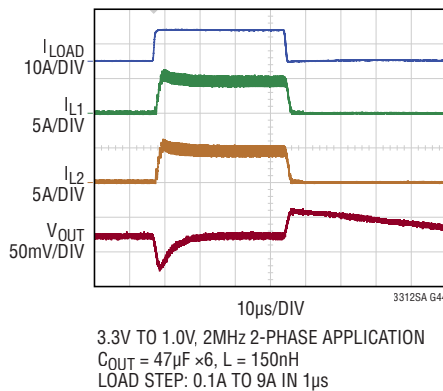
2-Phase Configuration Load Transient Response, Pulse-Skipping Mode
