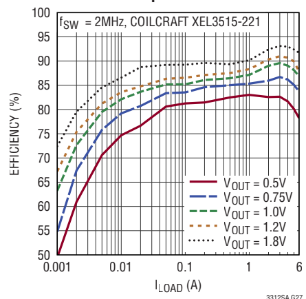
Efficiency, V_{IN} = 5.0\text{V} , Burst Mode Operation
