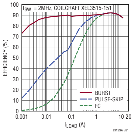
2-Phase Efficiency vs Load, 2.5V to 1.0V, f_{\text{SW}} = 2\text{MHz}
