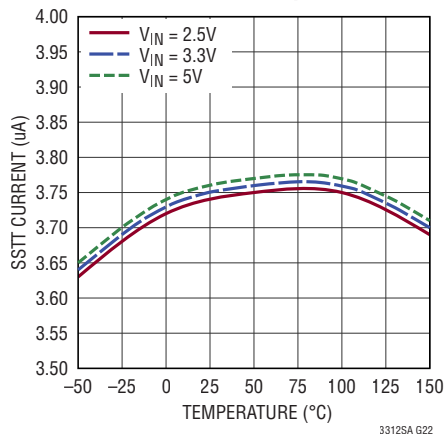
SSTT Current vs Temperature
