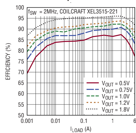
Efficiency, V_{IN} = 2.5\text{V} , Burst Mode Operation
