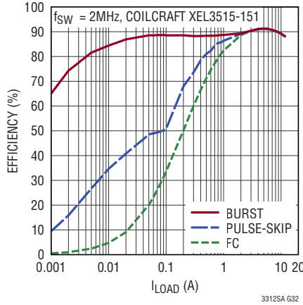
2-Phase Efficiency vs Load, 3.3V to 1.0V, f_{\text{SW}} = 2\text{MHz}
