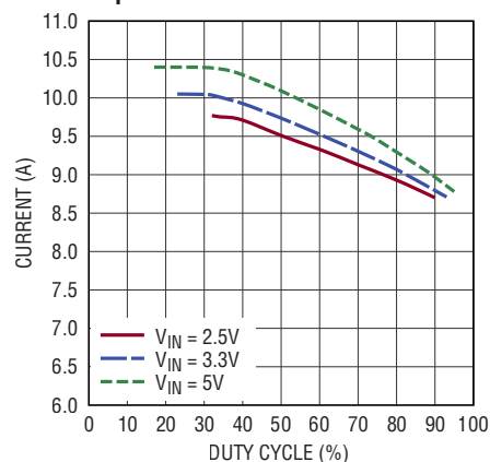
Top Switch Current Limit
