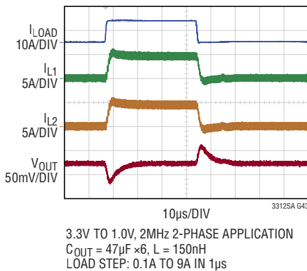
2-Phase Configuration Load Transient Response, Forced Continuous Mode
