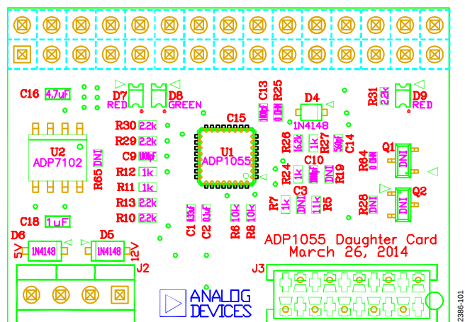
Figure 102. PCB Assembly, Top
