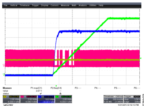
Figure 29. Demonstration of Overshoot Protection at No Load Green Trace: Output Voltage Blue Trace: Input Voltage Red Trace: PWM
