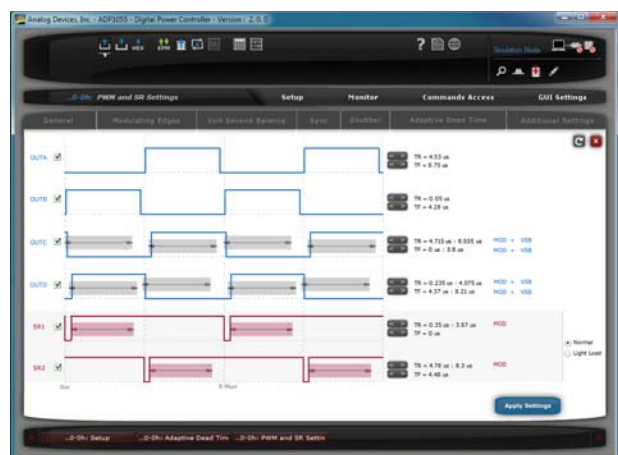
Figure 19. PWM and SR Window (Full Bridge Phase Shifted)
