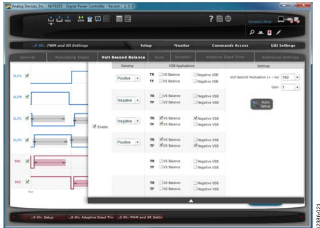
Figure 21. PWM and SR Window (Full Bridge Phase Shifted)
