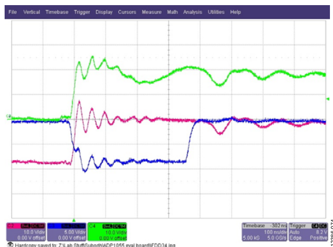
Figure 75. Active Clamp Snubber Enabled, Zoomed In, 10 A Load 50 ns Delay, 380 ns Snubber on Time Green Trace: Drain—Source Voltage of Low Side SR FET Blue Trace: Gate—Source Voltage of Snubber FET Red Trace: Drain—Source Voltage of Snubber FET
