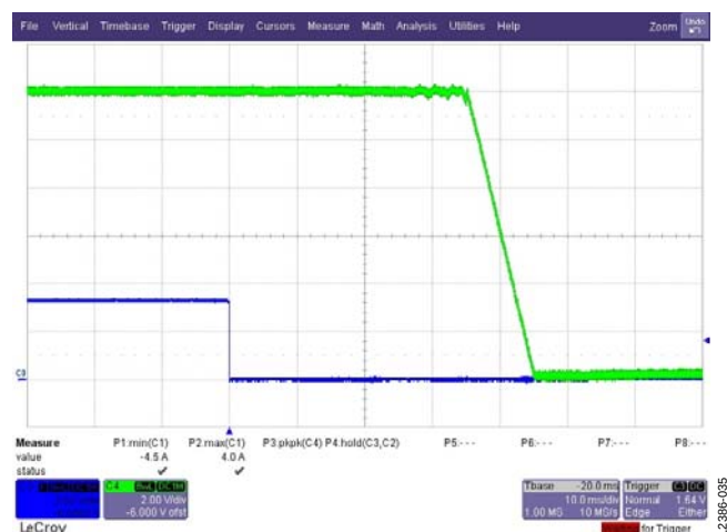
Figure 35. Soft Stop from Light Load Mode Green Trace: Output Voltage Blue Trace: Hardware PSON
