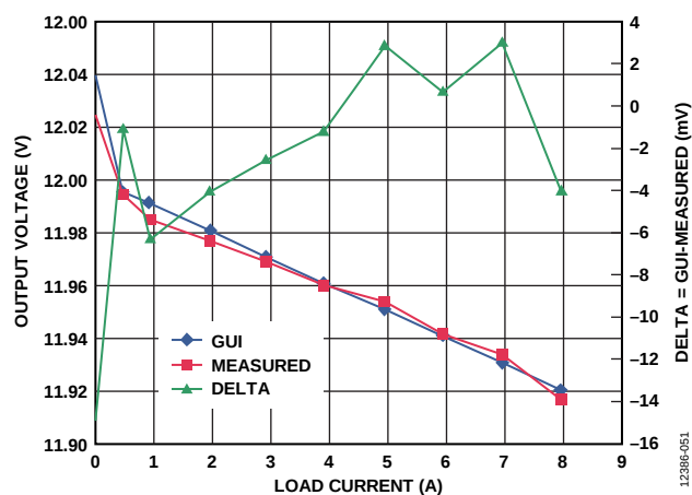
Figure 52. VOUT_DROOP = 10 mV/A
