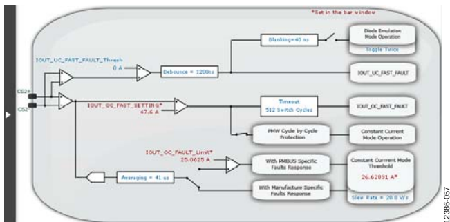
Figure 58. Additional Settings in IOUT Window
