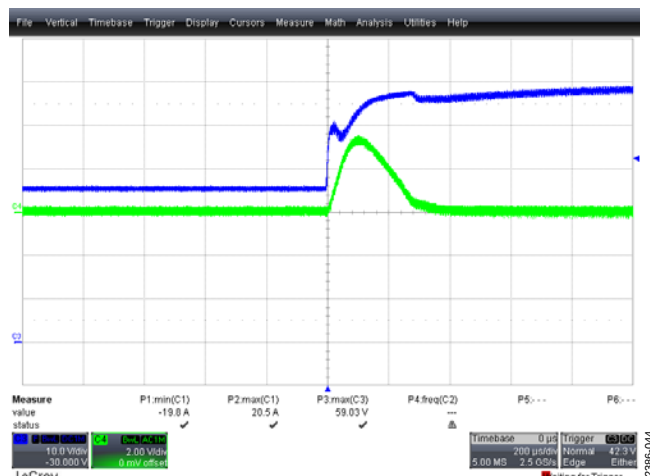
Figure 44. Line Voltage Feedforward DISABLED, 5 A Load Green Trace: AC Coupled Output Voltage Blue Trace: Input Voltage
