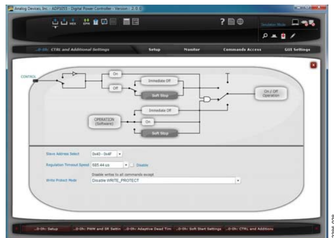
Figure 28. PSON Window
