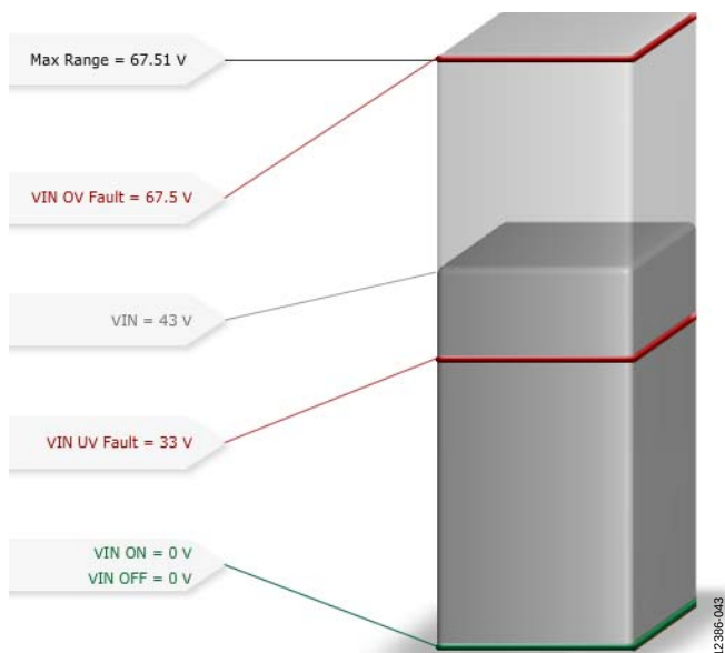
Figure 43. VIN Window
