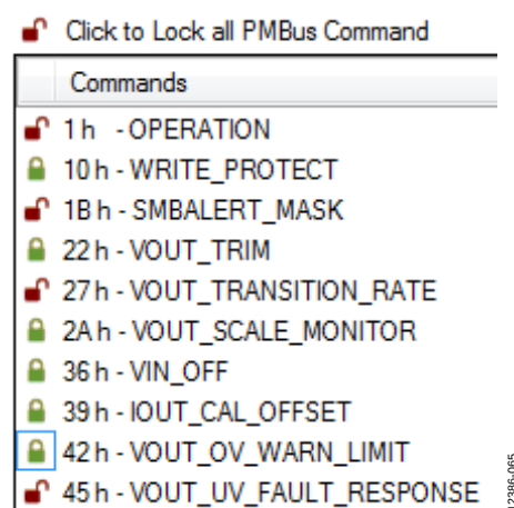
Figure 66. Sample Command Masking Window
