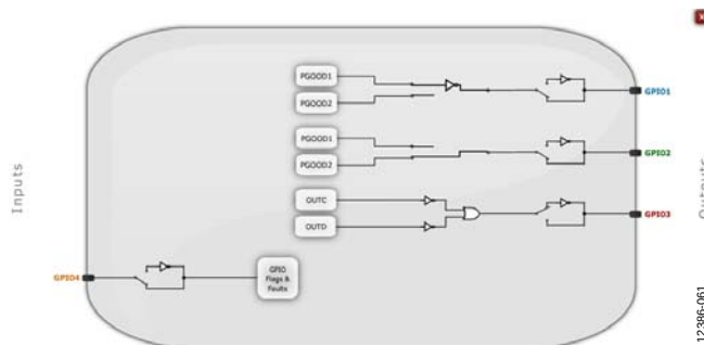
Figure 62. GPIO Window
