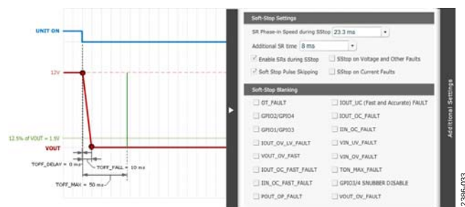
Figure 33. Soft-Stop Window
