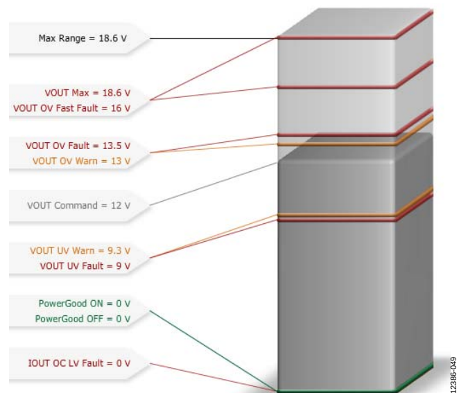
Figure 50. VOOUT Window
