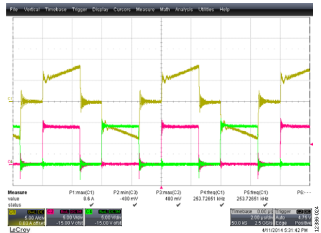
Figure 24. Volt Second Balance Enabled, Duty Balance Disabled Yellow Trace: Primary Current, 5 A/Div Red and Green Trace: OUTB and OUTD
