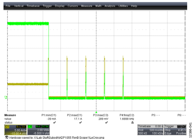
Figure 41. IOUT_OC_FAULT under Short-Circuit Fault Response Set to Shut Down and Retry 4 Times Green Trace: Output Voltage Yellow Trace: Load Current
