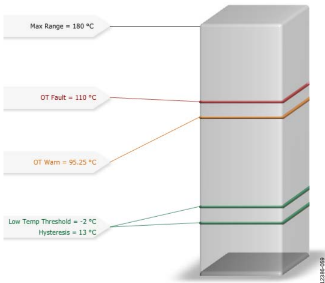
Figure 60. Temperature Window
