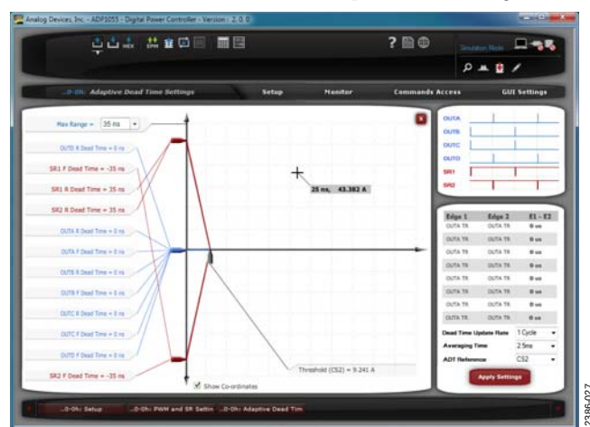
Figure 27. ADT Window
