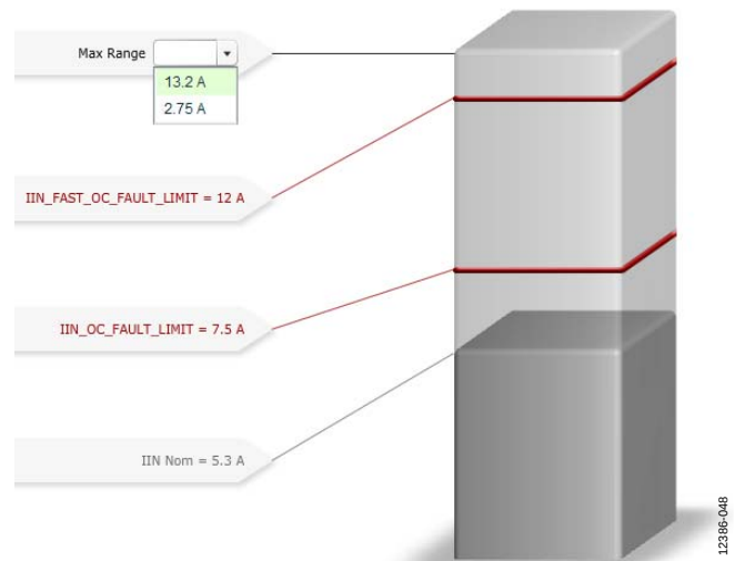
Figure 49. IIN Window
