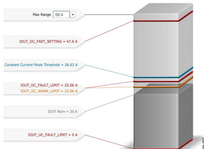
Figure 54. IOUT Window
