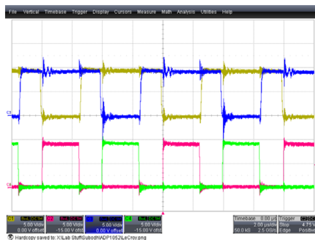
Figure 20. PWM Example Under 10 A Load Top 2 Waveforms: SR1 and SR2 Bottom 2 Waveforms: OUTB and OUTD
