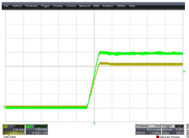
Figure 57. Constant Current Mode in a Load Resistor Green Trace: Output Voltage Yellow Trace: Load Current
