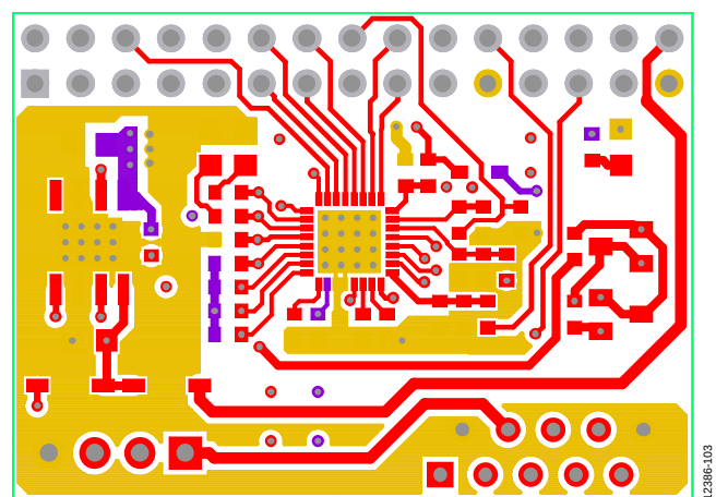
Figure 104. PCB Layout, Top Layer
