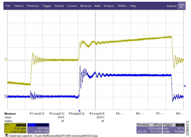
Figure 72. Active Clamp Snubber Enabled, Zoomed In, 20 A Load Yellow Trace: Primary Current Blue Trace: Drain Source Voltage of Low Side SR FET
