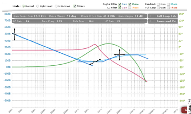
Figure 77. Digital Filter Settings Window
