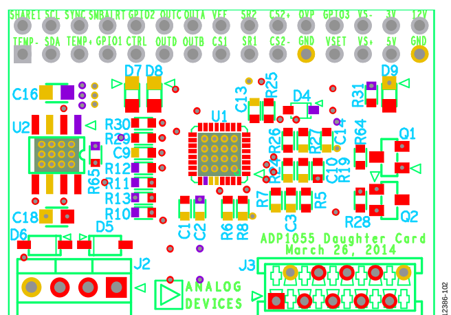
Figure 103. PCB Layout, Silkscreen Layer Top
