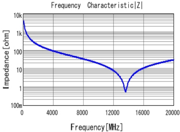
■ GJM0335C1ER40WB01 |Z| DC0V, 25degC
