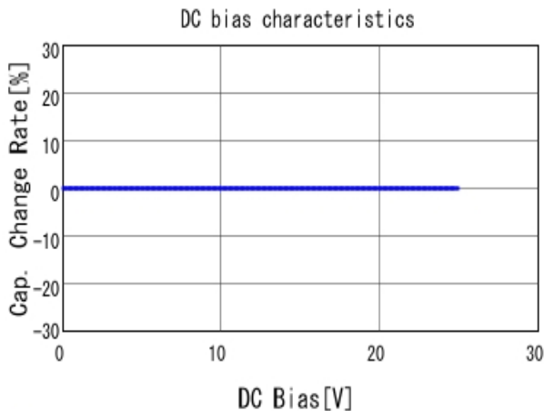
■ GJM0335C1ER40WB01 C-DC bias capchange, 25.0degC, AC1V
