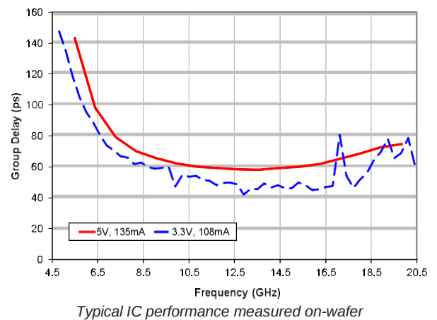
Group Delay
