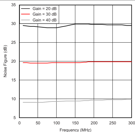
Figure 6-3. Noise Figure vs Frequency
