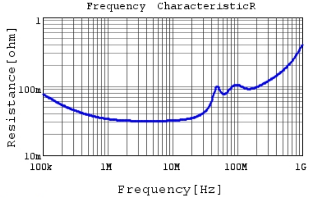
RDED72J104K5B1H03B R DC0V, 25degC
