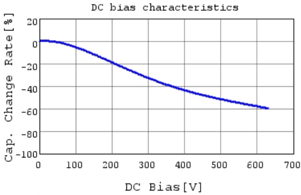
RDED72J104K5B1H03B C-DC bias capchange, 25.0
