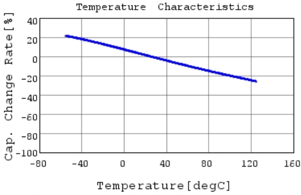
RDED72J104K5B1H03B C-Temp. capchange, DCOV,
