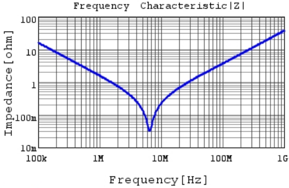
RDED72J104K5B1H03B |Z| DC0V, 25degC
