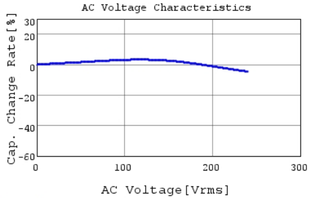
RDED72J104K5B1H03B C-AC Voltage capchange, I
