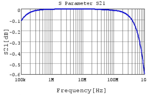
RDED72J104K5B1H03B S21 DCOV, 25degC
