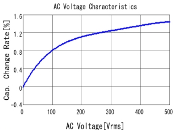
■ DE11XRA470KA4BQ01F C-AC Voltage capchange, DC0V, 20.0
