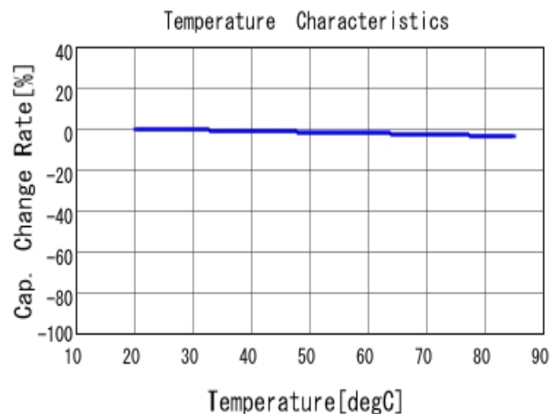
■ DE11XRA470KA4BQ01F C-Temp. capchange, DC0V, AC1Vrms
