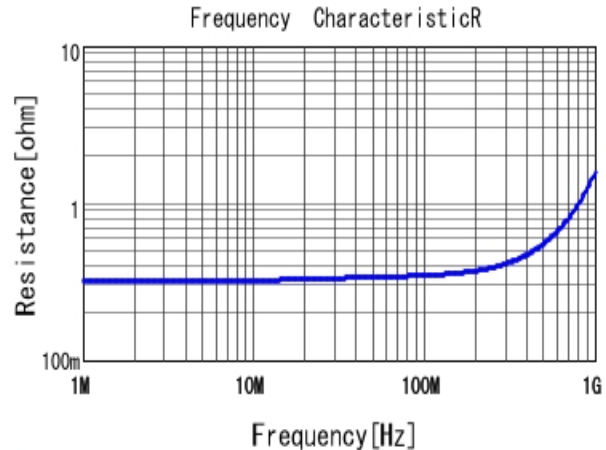
■ DE11XRA470KA4BQ01F R DC0V, 20degC
