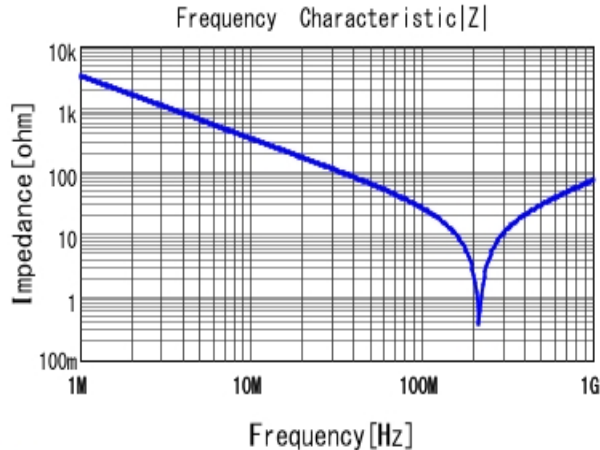
■ DE11XRA470KA4BQ01F |Z| DC0V, 20degC
