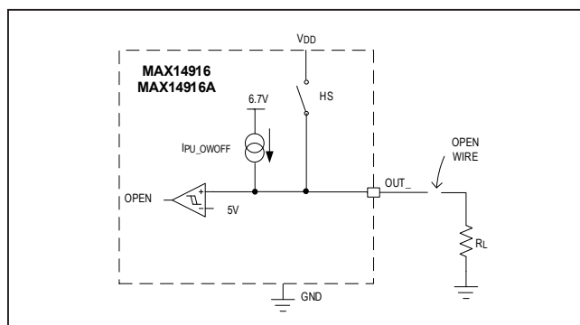
Figure 5. Open-Wire Detection Scheme
