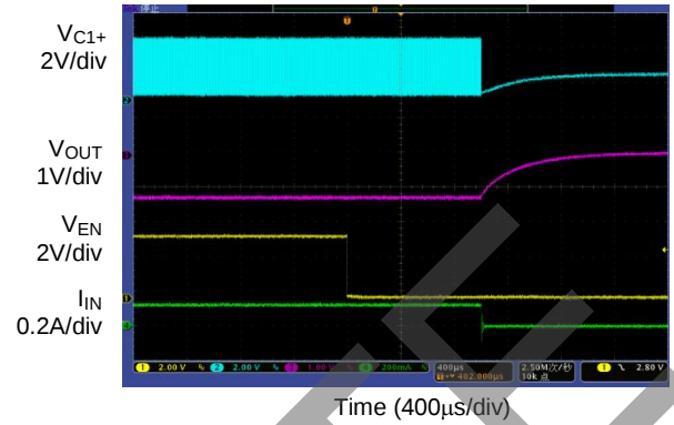
1.5x Mode Turn off Characteristic
