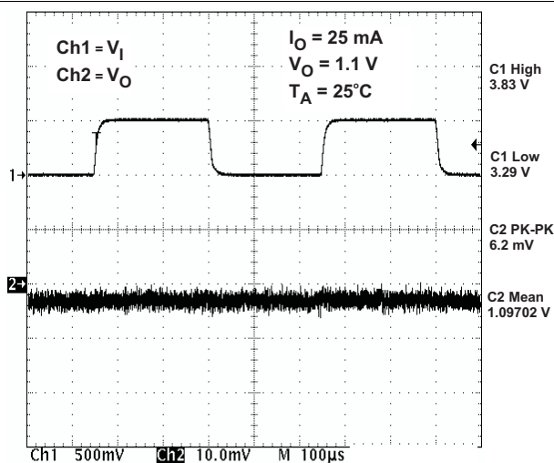
Figure 23. LDO1 Line Transient Response
