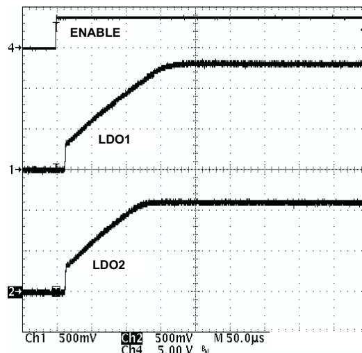
Figure 22. Start-up LDO1 and LDO2
