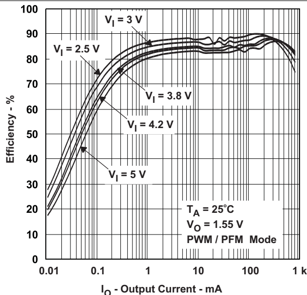
Figure 39. DCDC3 Efficiency
