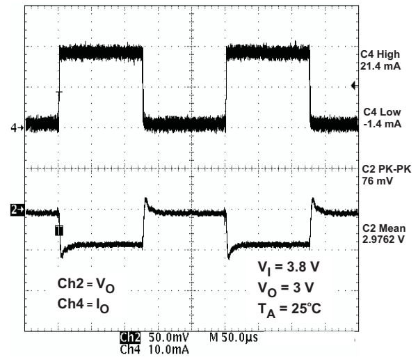
Figure 28. VRTC Load Transient Response
