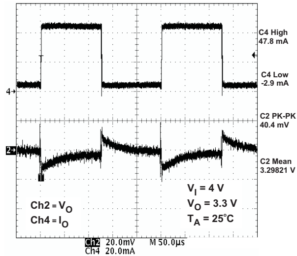
Figure 27. LDO2 Load Transient Response
