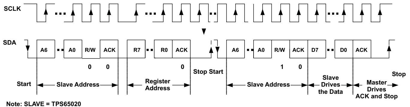
Figure 34. Serial I/F READ from TPS65021: Protocol B
