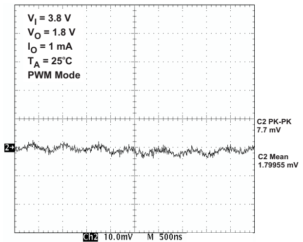
Figure 20. VDCDC2 Output Voltage Ripple
