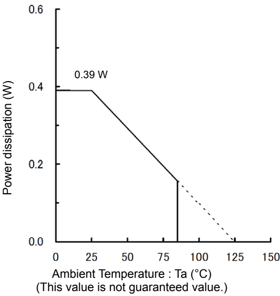
Figure 14. Power dissipation Pd [W]
