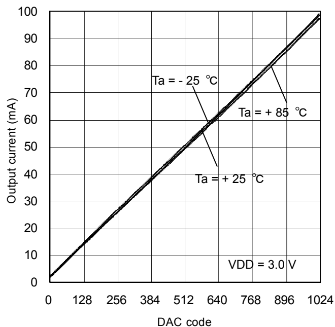
Figure 6. Output current vs. DAC code
