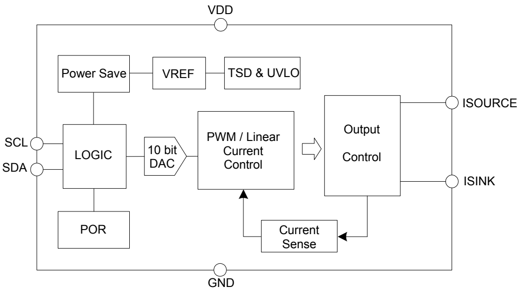
Figure 3. Block diagram
