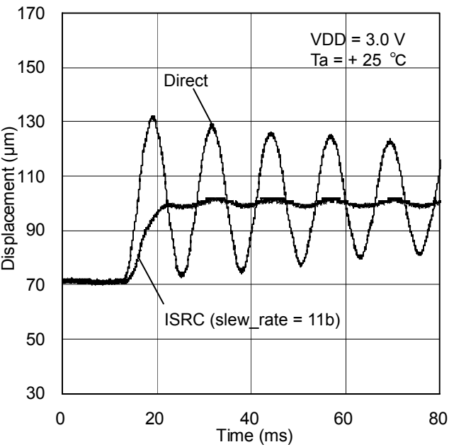
Figure 10. Displacement vs. settling time (slew_rate = 11b)
