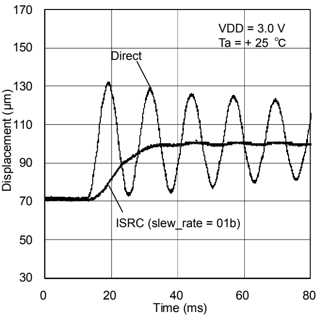
Figure 8. Displacement vs. settling time (slew_rate = 01b)
