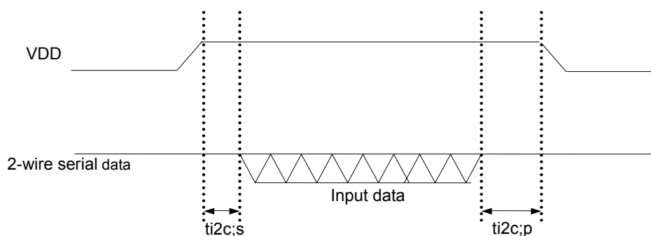
Figure 13. Timing Waveform Applying Power (VDD) Until Input of Serial Data
