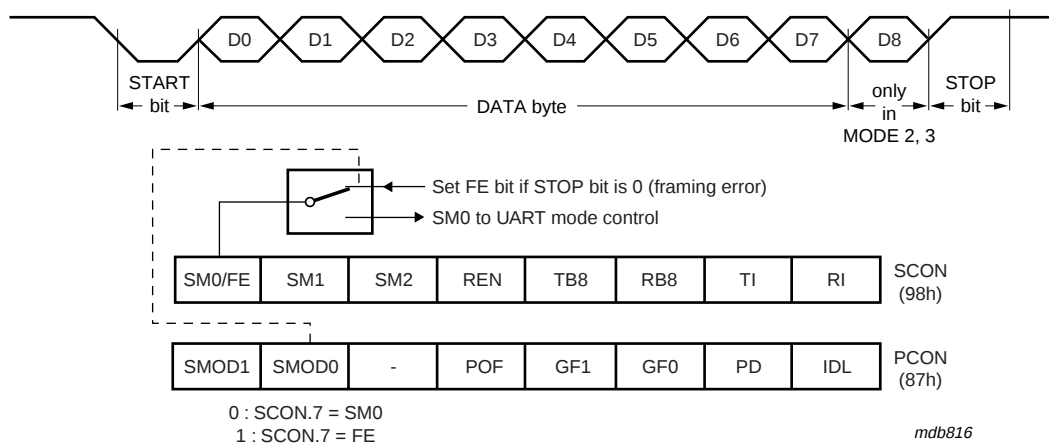
Fig 6. UART framing error detection
