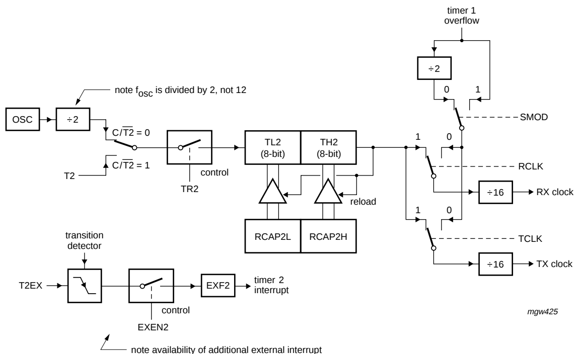
Fig 5. Timer 2 in baud rate generator mode
