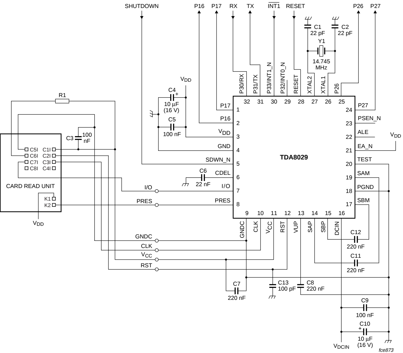
Fig 14. Application diagram
