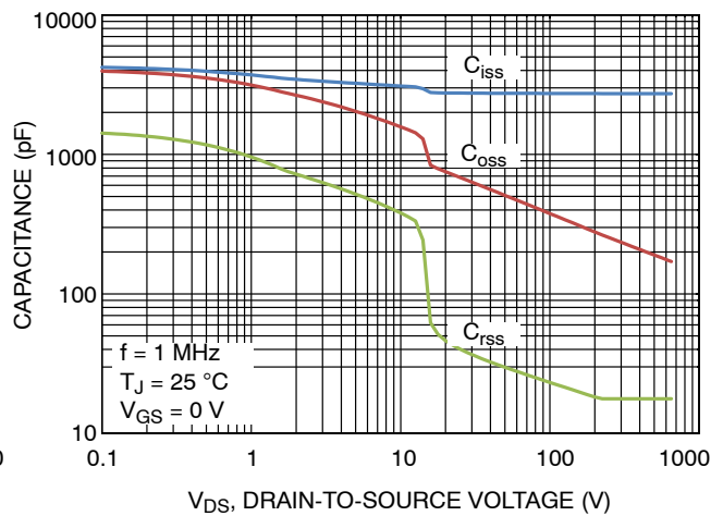
Figure 10. Capacitance Characteristics
