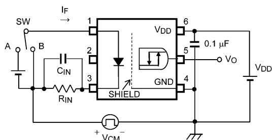
Fig. 12.1.6 Common-Mode Transient Immunity Test Circuit and Waveform
