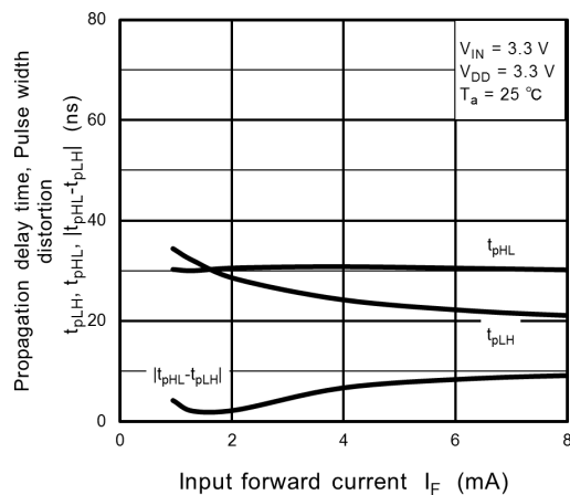
Fig. 12.2.12 t_{pHL} , t_{pLH} , |t_{pHL} - t_{pLH}| - I_F
