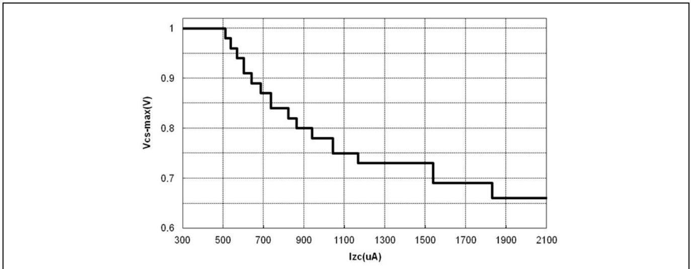
Figure 8 V_{CS\_max} versus I_{ZC}
