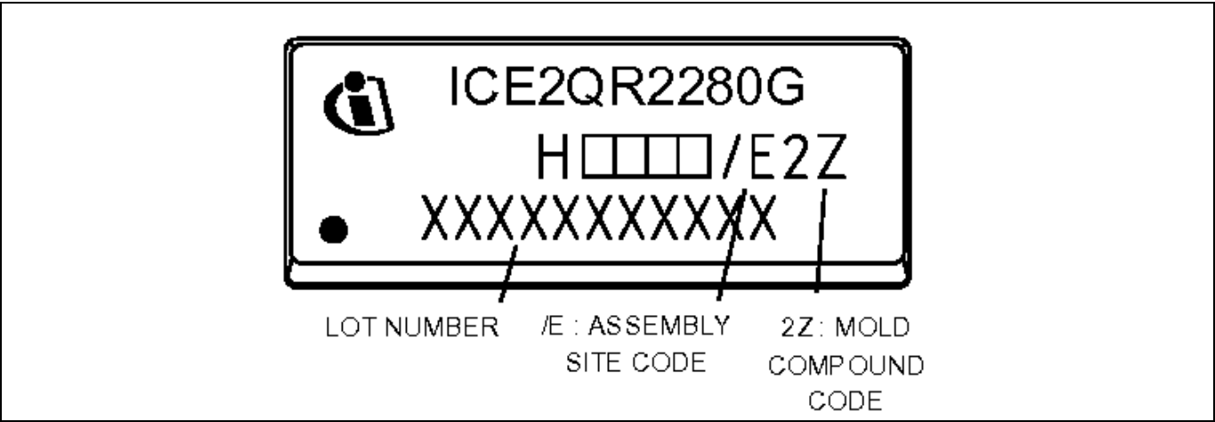
Figure 16 Marking for ICE2QR2280G
