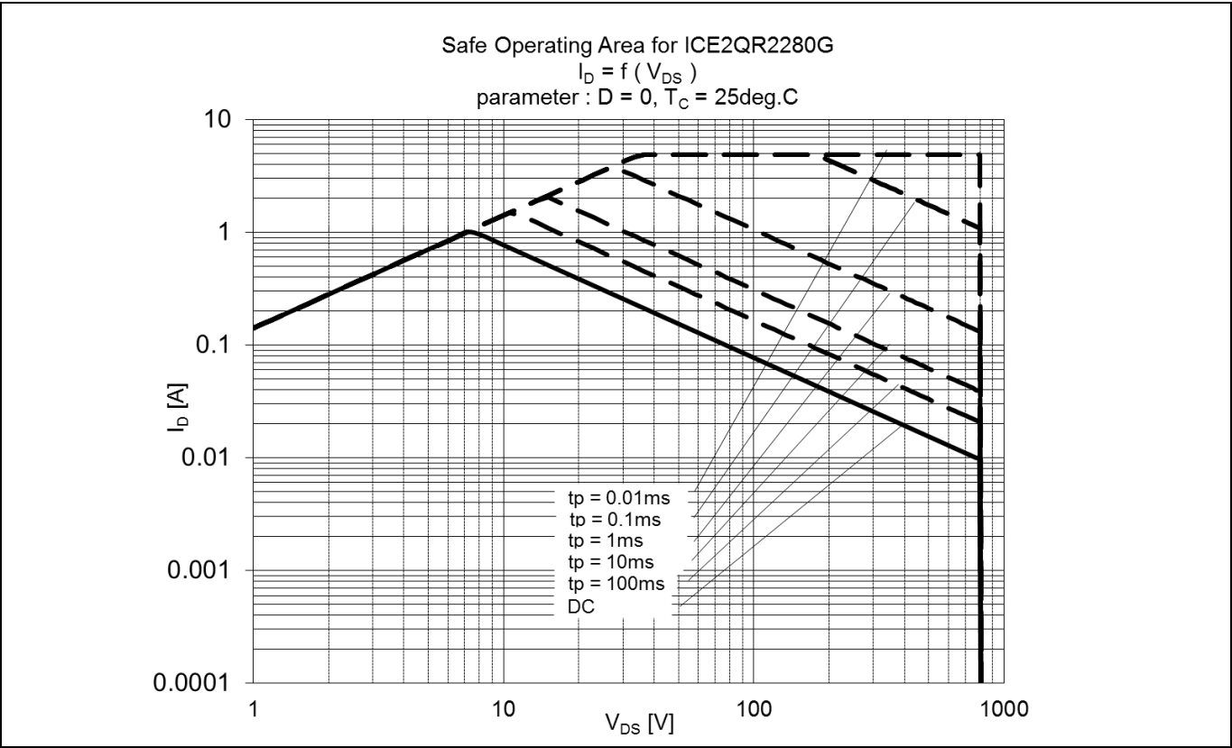
Figure 10 Safe Operating Area (SOA) curve for ICE2QR2280G
