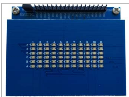
Figure 1: Photo of IS31FL3743B Evaluation Board
