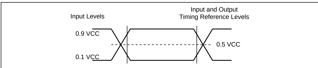
Figure 58. AC Measurement I/O Waveform
