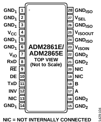
Figure 11. ADM2861E/ADM2865E Pin Configuration
