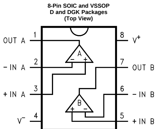
Pin Functions
