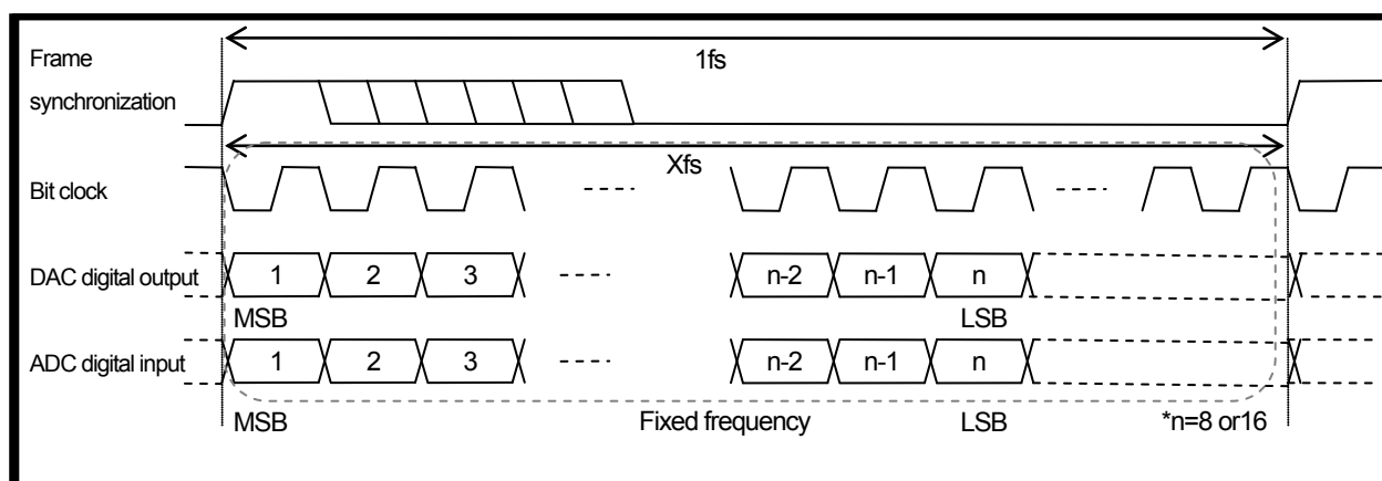
Figure 4-20 Bit clock of a fixed frequency
