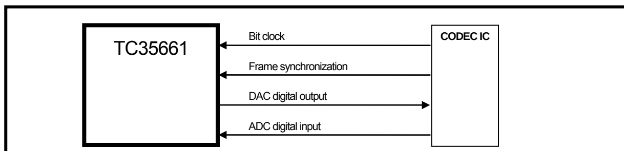
Figure 4-8 CODEC connection example (TC35661 is Slave.)
