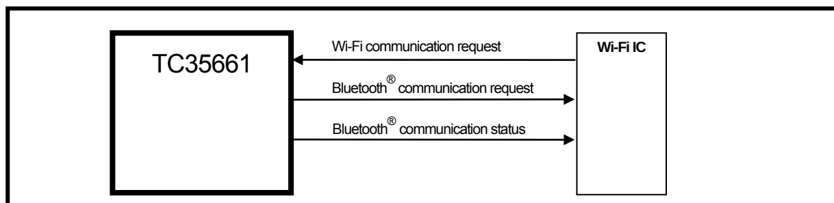
Figure 4-33 Connection example of 3-wire
