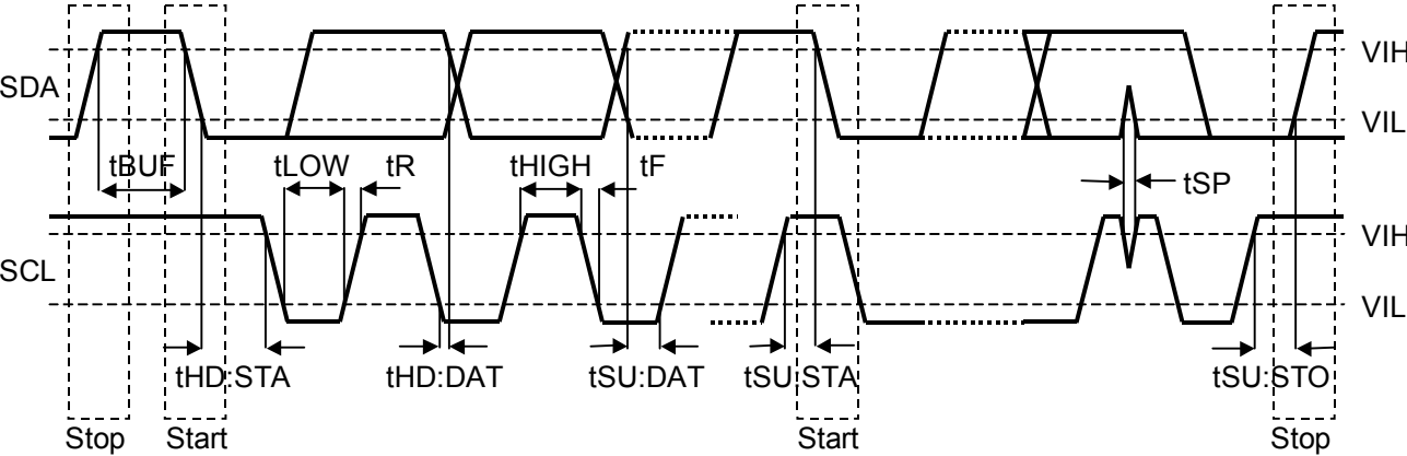
Figure 6. I²C Bus mode Timing
