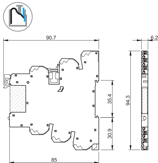
39.60/39.60.3 39.61/39.61.3 Push-in terminal
