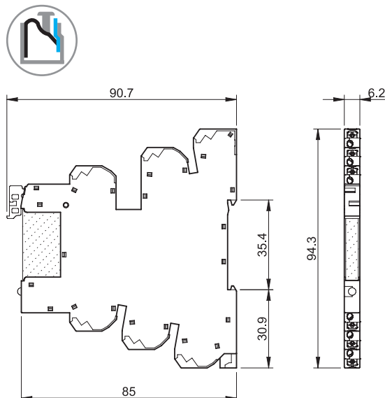
39.70 39.71 Push-in terminal
