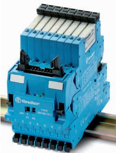
Connected MasterADAPTER
