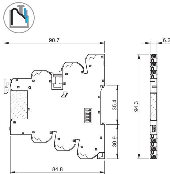
39.90 39.91 Push-in terminal
