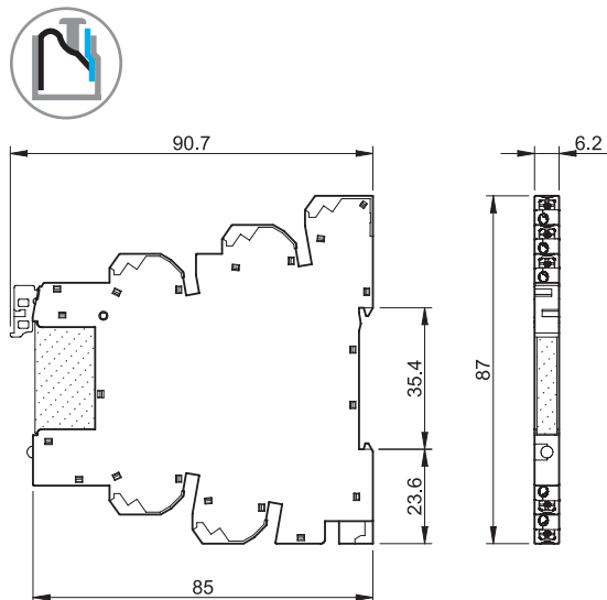
39.00/39.01 39.50/39.51 Push-in terminal
