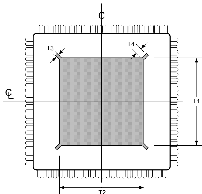
Figure 30. ePad Diagram
