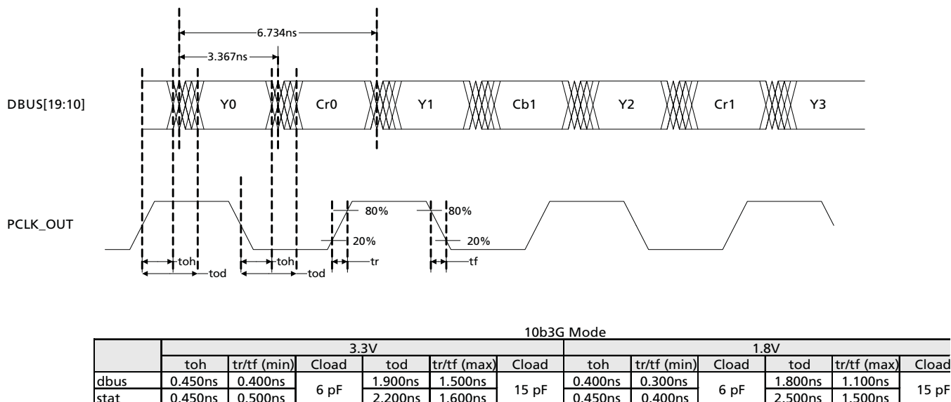
Figure 4-6: PCLK to Data and Control Signal Output Timing - DDR Mode
