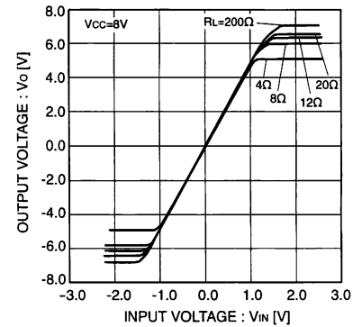
Fig.21 Load fluctuation I/O characteristic ch3 (Ta=85°C)
