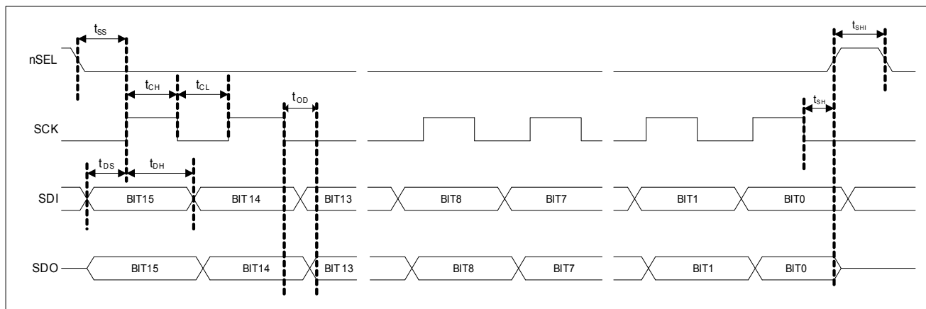
Figure 3. Timing Diagram
