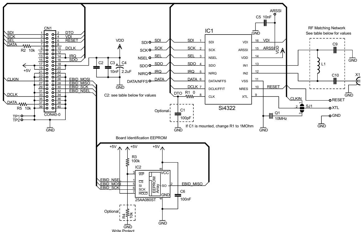
Figure 13. Schematic
