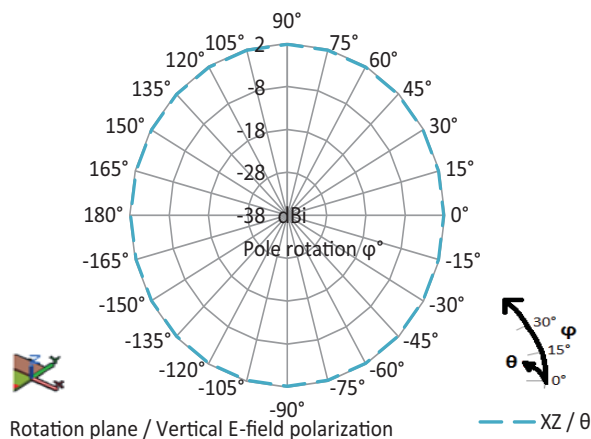
Fig. 6 - VJ5601M915MXBSR XZ Radiation Pattern
