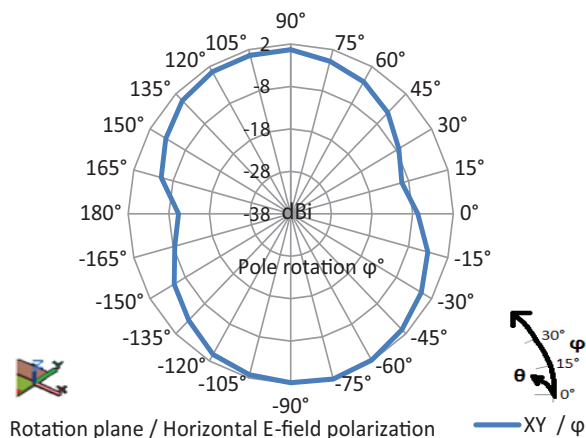
Fig. 4 - VJ5601M915MXBSR XY Radiation Pattern
