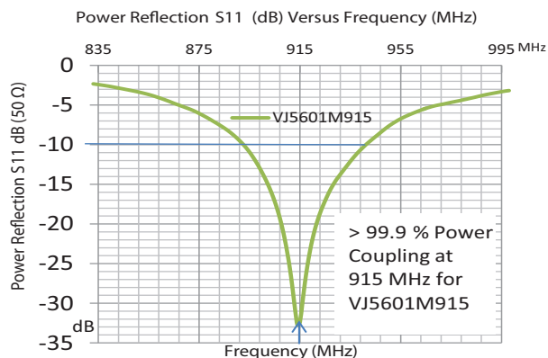
Fig. 2 - VJ5601M915 Tuned to 915 MHz with > 99.9 % Power Coupled
