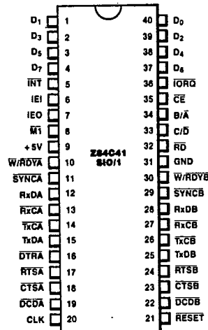
Figure 4. 40-pin Dual-In-Line Package (DIP), Pin Assignments
