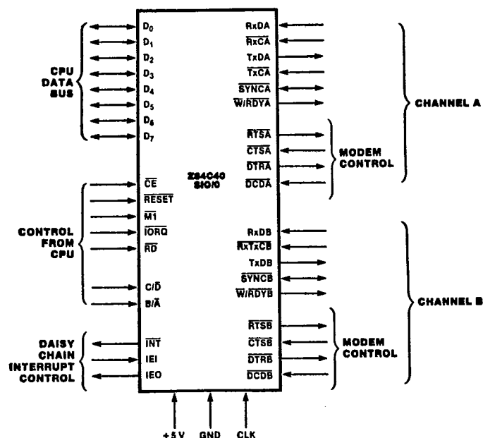
Figure 5. Pin Functions
