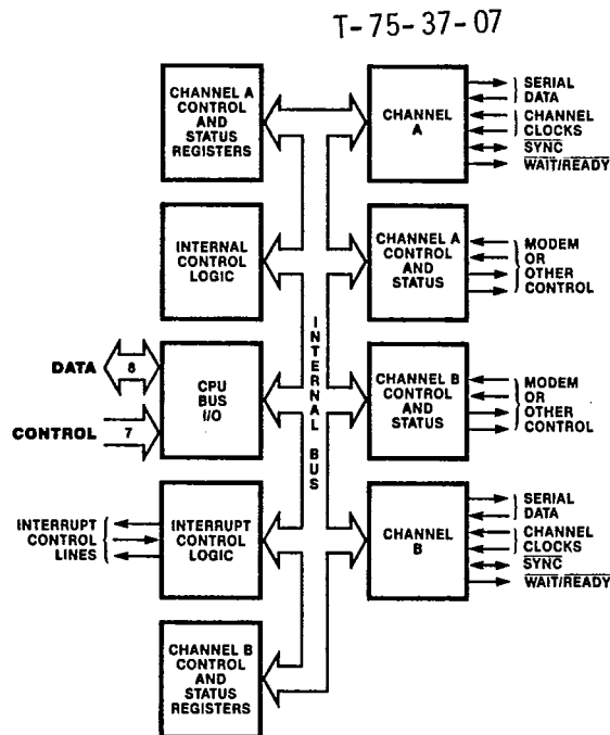
Figure 8. Block Diagram
