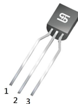
1: Collector 2: Base 3: Emitter
