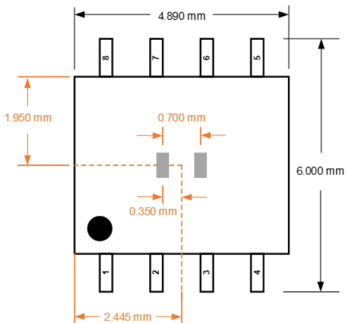
Figure 23: XtremeSense TMR Current Sensor Location in x-y Plane for CT453 in SOIC-8 Package
