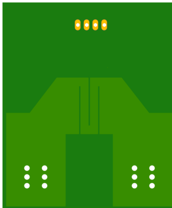
Figure 22: Recommended PCB Layout (Bottom Layer) for CT453
