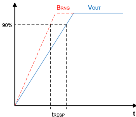
Figure 19: CT453 Response Time Curve
