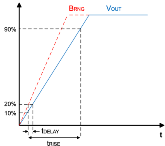
Figure 20: CT453 Propagation Delay and Rise Time Curve
