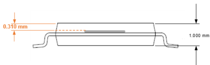
Figure 26: XtremeSense TMR Current Sensor Location in z Dimension for CT453 in TSSOP-8 Package
