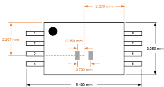
Figure 25: XtremeSense TMR Current Sensor Location in x-y Plane for CT453 in TSSOP-8 Package
