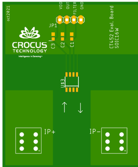
Figure 21: Recommended PCB Layout (Top Layer) for CT453
