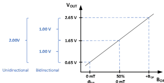
Figure 13: Linear Output Voltage Range (OUT) vs. Measured Magnetic Field ( B_{OP} )
