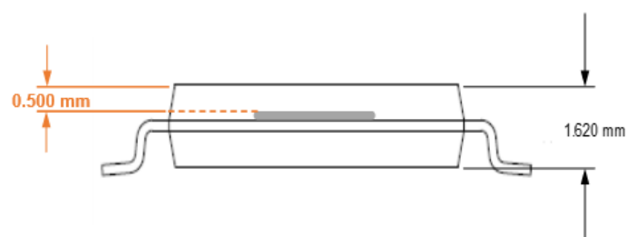
Figure 24: XtremeSense TMR Current Sensor Location in z Dimension for CT453 in SOIC-8 Package
