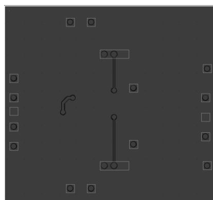
Fig. 6: Layout - Bottom
