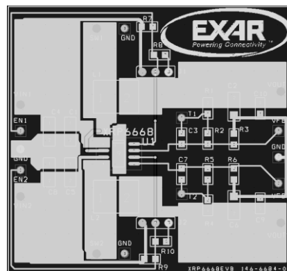
Fig. 4: Component Placement 2 – Top Side
