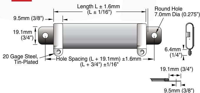
Fig. 5 With Low Profile Axial Tabs (H1)
