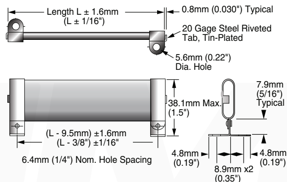
Fig. 6 With Standoff Axial Tabs (H2)
