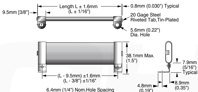
Fig. 3 With Right Angle Radial Tabs – same direction – (G2)
