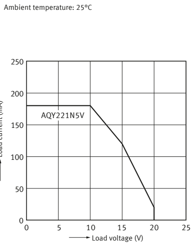
2-2. Load current vs. load voltage characteristics
