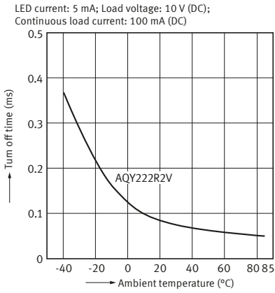
4-1. Turn off time vs. ambient temperature characteristics
