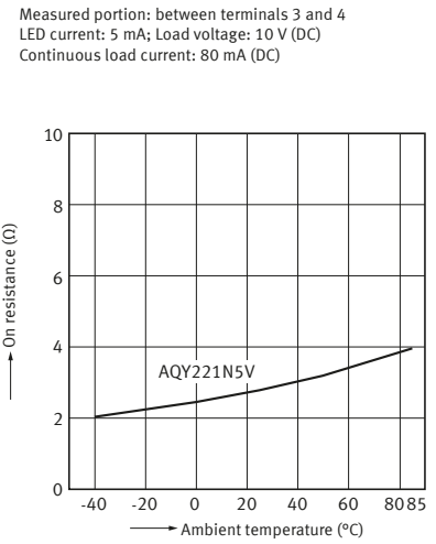
3-2. On resistance vs. ambient temperature characteristics
