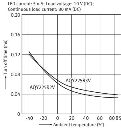
4-2. Turn off time vs. ambient temperature characteristics
