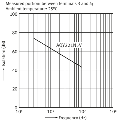
14-2. Isolation vs. frequency characteristics ( 50 Ω impedance )
