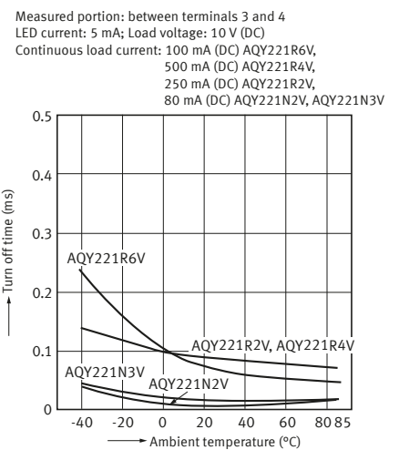
5-1. Turn off time vs. ambient temperature characteristics
