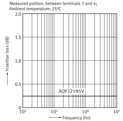
15-2. Insertion loss vs. frequency characteristics ( 50 Ω impedance )
