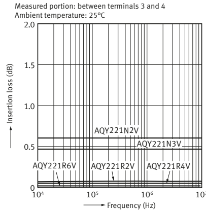
15-1. Insertion loss vs. frequency characteristics ( 50 Ω impedance )
