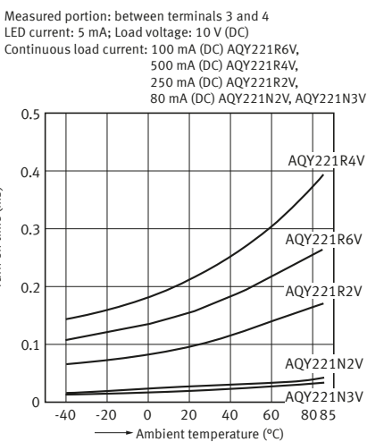
4-1. Turn on time vs. ambient temperature characteristics
