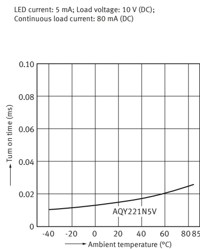
4-2. Turn on time vs. ambient temperature characteristics
