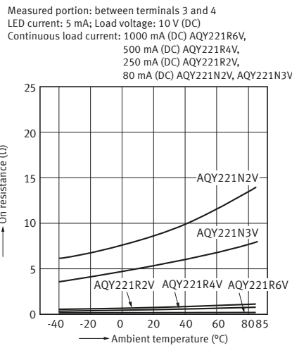
3-1. On resistance vs. ambient temperature characteristics
