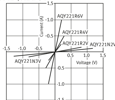
9-1. Current vs. voltage characteristics of output at MOS portion
