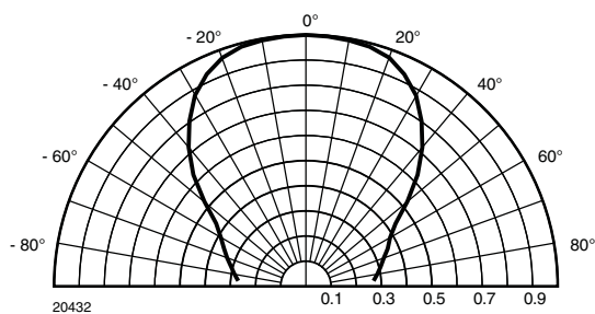
Fig. 12 - Directivity
